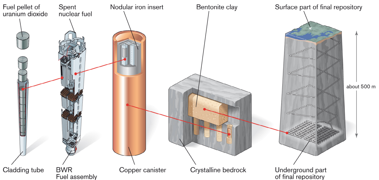
Figure 4.1: Disposal of spent fuel according to the Swedish/Finnish KBS-3 method (SKB)
