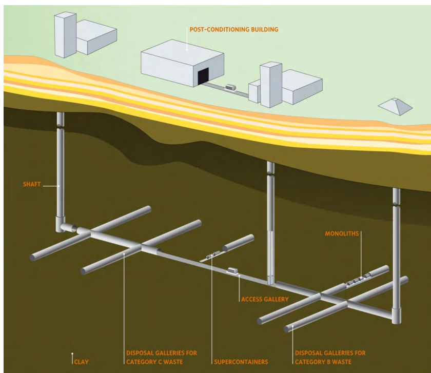
Figure 5.3: Illustration of geological repository concept (Courtesy NIRAS/ONDRAF)
