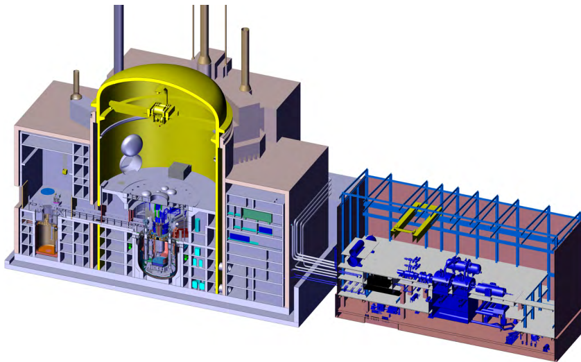
Figure 4.3: View of the ASTRID technological demonstration plant (fast neutron reactor) (©CEA)
