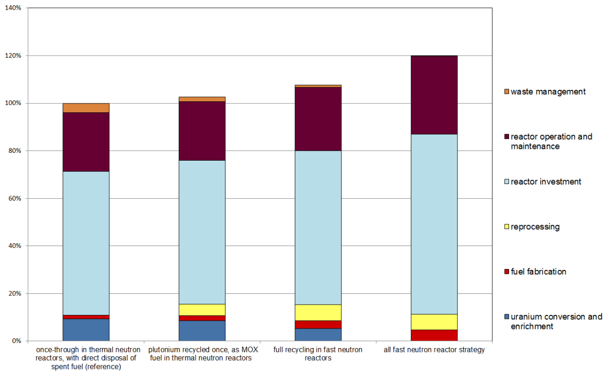
Figure 5.5: Relative cost estimates for alternative types of fuel cycles (courtesy NEA)
