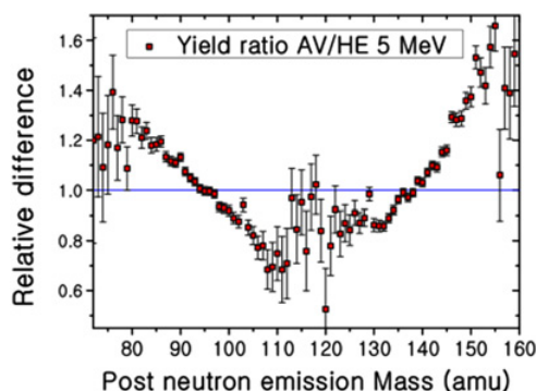
Figure 1. Relative difference between the average correction of prompt neutron multiplicity and a correction introducing higher neutron multiplicities for the heavy fragment only.
