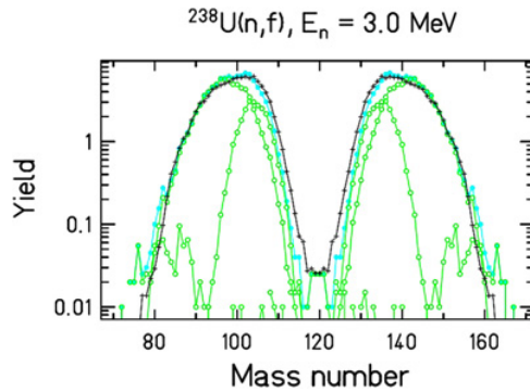
Figure 3. Mass distribution of ^{238}\text{U} ( n,f ) at 3 MeV incident neutron energy. Experimental data (black dots), GEF code calculation (blue dots) and mode separation (green dots).
