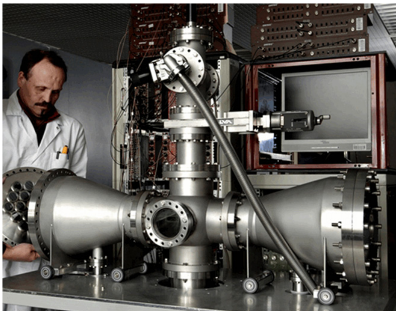
Figure 4. Photo of the VERDI 2v-2E spectrometer under construction at the Joint Research Centre -IRMM.
