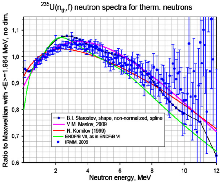
Figure 2. The most recent prompt fission neutron spectrum measurement compared to literature and relevant evaluations [13].
