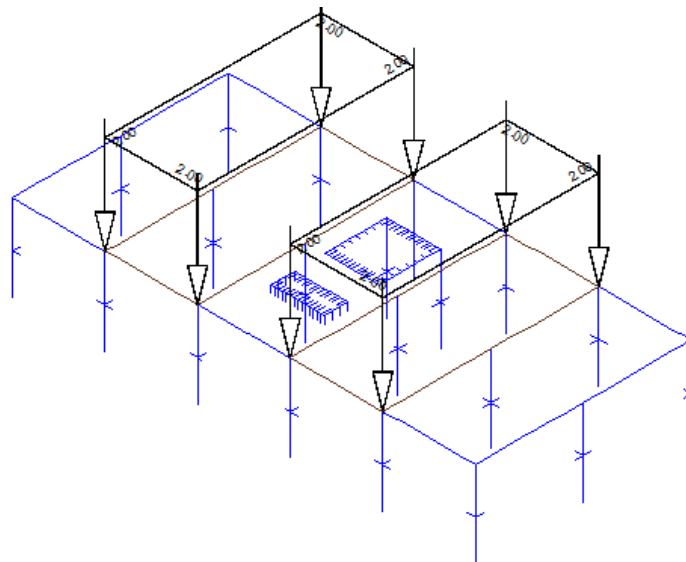
Fig.2.2.11 – Arrangement of the loads for load case 1366 (values in kN/m)
