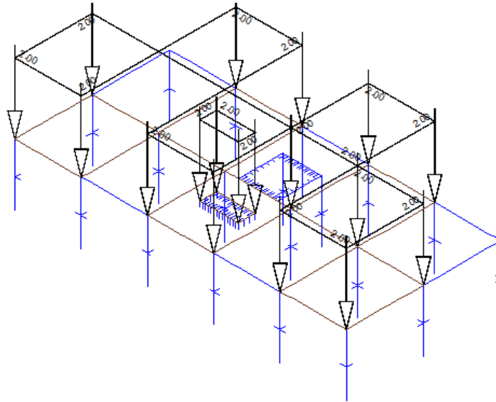
Fig.2.2.10 – Arrangement of the loads for load case 1356 (values in kN/m)
