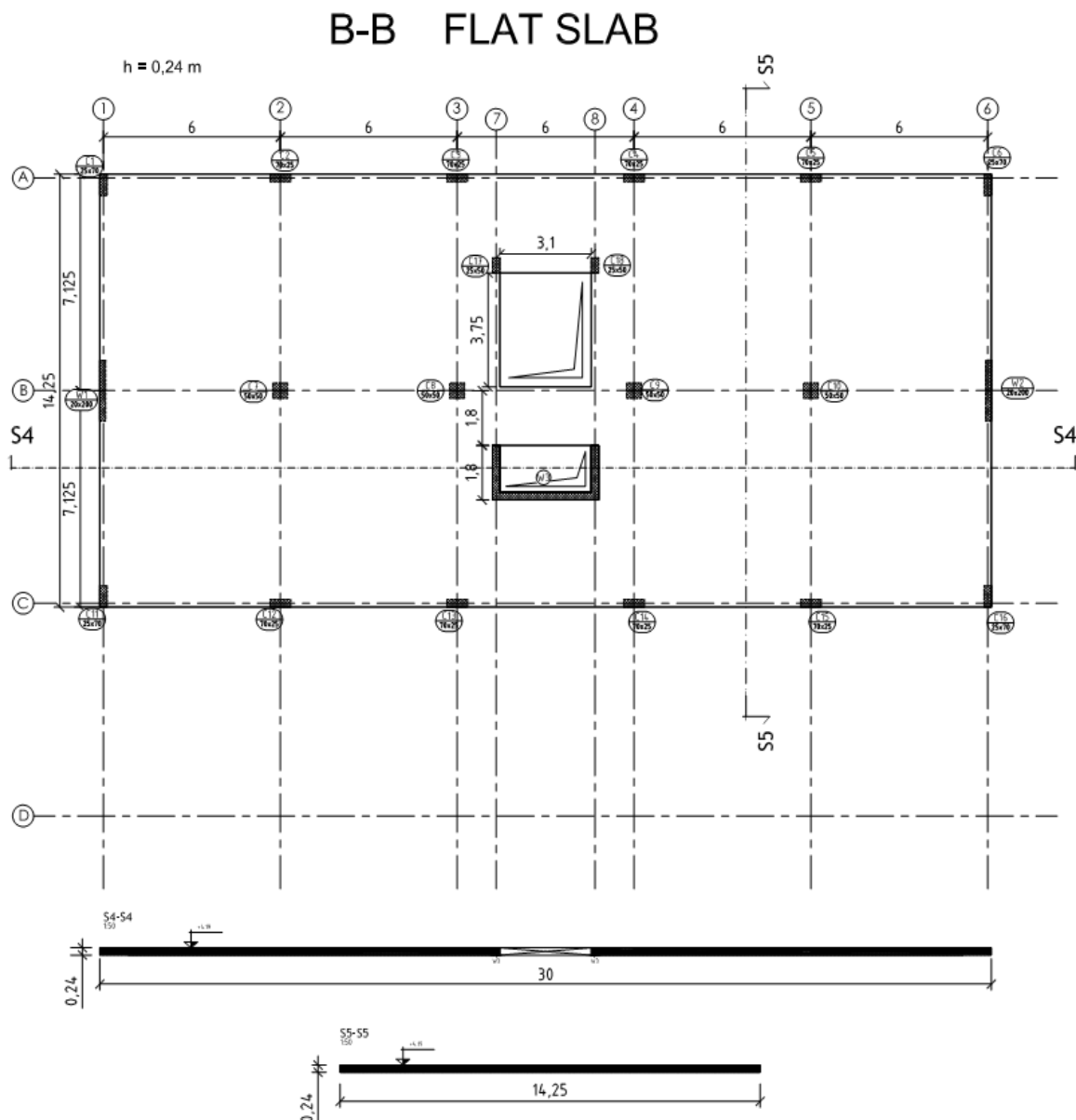
Fig.1.2.5 Flat Slab h = 0,24 \text{ m}
