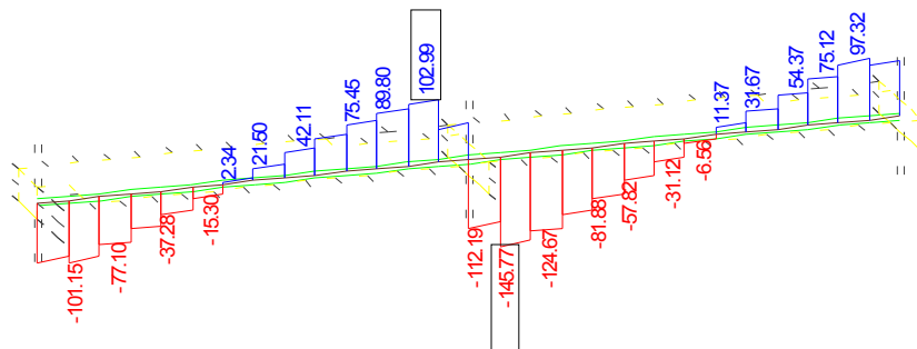
Fig.2.3.10 Values for V_z for the superposition of “min V_z ”
