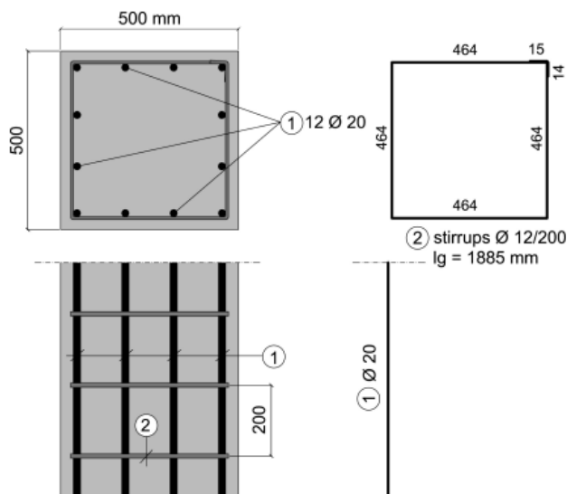
Fig. 6.2.11 Layout of the reinforced column B2
