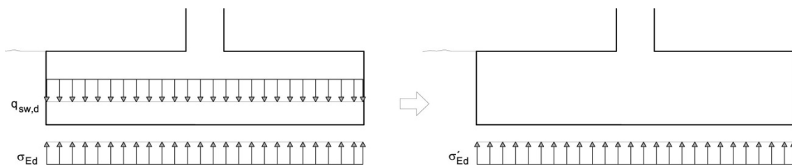
Fig.4.2.3 Effective pressure
