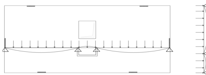
Fig.1.2.2 Peripheral walls
