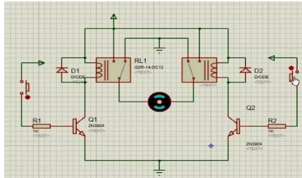
Figure 9. Diagram of the H-bridge that controls a motor [16].
