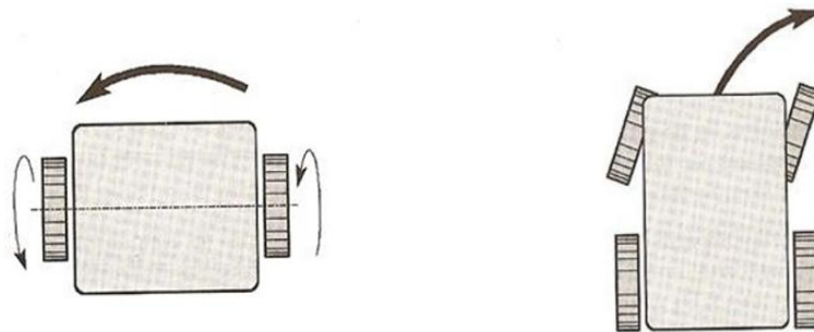
Figure 6. Rotation in differential configuration (left) and Ackerman configurations (right) [11].
