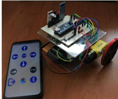
Figure 4. EcateBot and Android control application [9].
