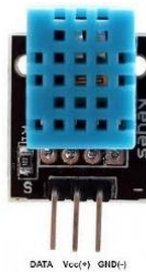
Figure 10. DHT11 sensor [13].
