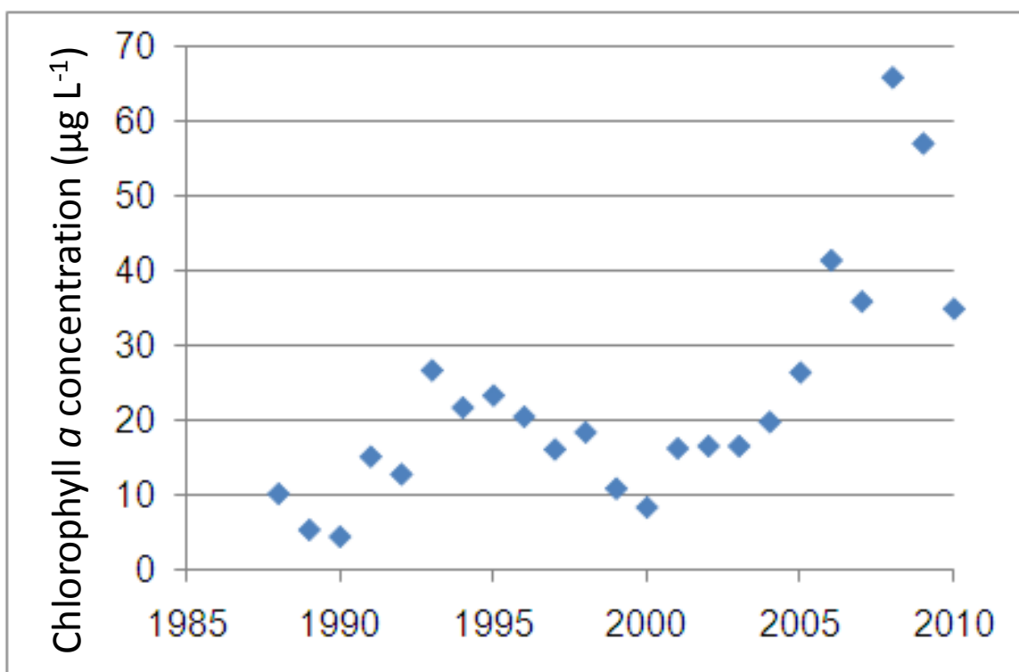
Figure 2.3 Open water chlorophylla concentrations in Loch Fitty, 1988-2010.
