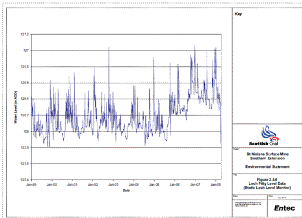
Figure 2.7 Loch Fitty water level, 1989 – 2008 (after SCCL, 2010c). (NB values before Jan 2006 are considered to be unreliable.)
