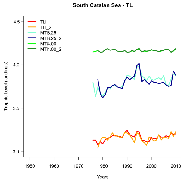
Fig. S2. Plots of TL of landed catch, MTI, TL of the surveyed community, and TL of the surveyed community when a TL > 3.25 cut-off was adopted (as for MTI) when model-generated annual TLs are used, compared to a single TL per species applied across the full time series (denoted as series 2 of each indicator in question) for the South Catalan Sea case study
