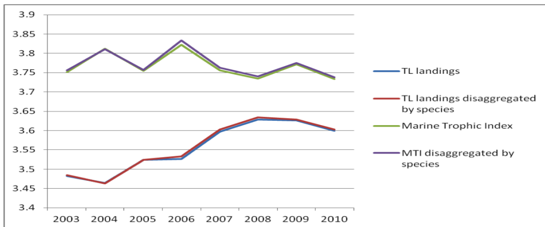
Fig. S3. Plot of TL of landed catch, and MTI (TL of landed catch with cut-off TL 3.25) in the Southern Benguela, for species-disaggregated TLs (modelled TL used for key, well described species, FishBase TLs for species falling into aggregated model groups) versus when an average TL was used for feeding guilds comprised of demersal fish and chondrichthyans other than deep- and shallow-water Cape hake and snoek. This comparison was made to verify usage of TL of the landed catch from 1950 onwards, since species-disaggregated data were not readily available until 2003
