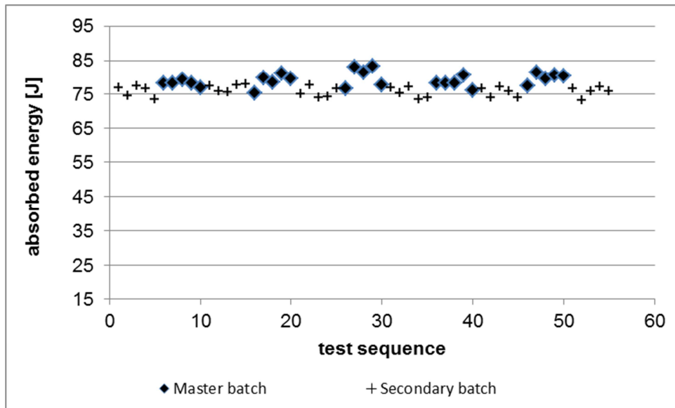
Figure 3: Absorbed energy values of 25 test pieces of ERM ® -FA015v, compared with 30 test pieces of ERM ® -FA015ab; data are displayed in the actual test sequence
