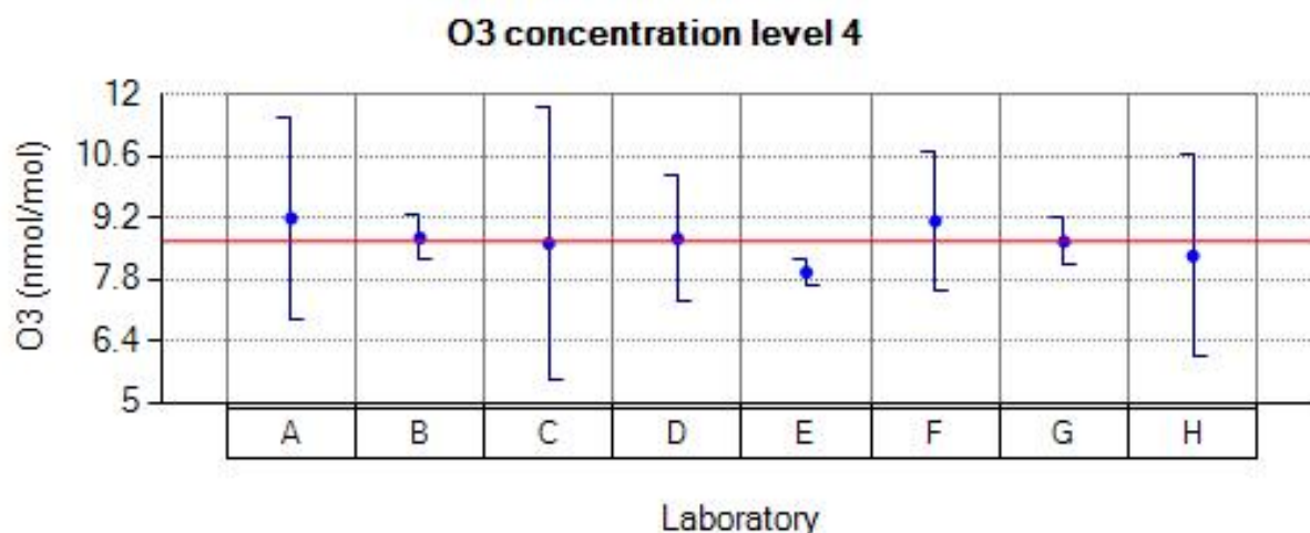
Figure 29: Reported values for O 3 run 4.
