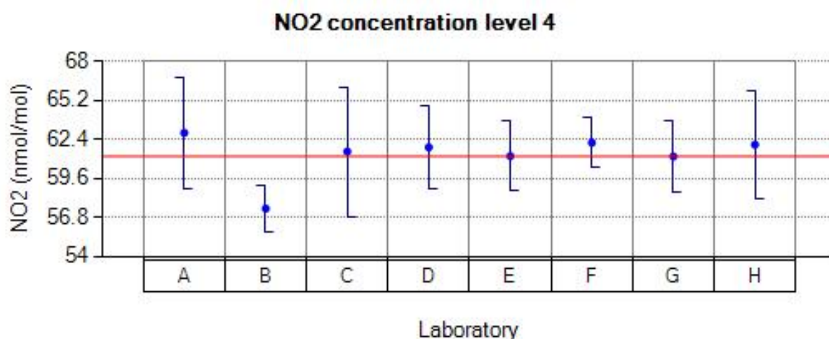
Figure 44: Reported values for NO 2 run 4.
