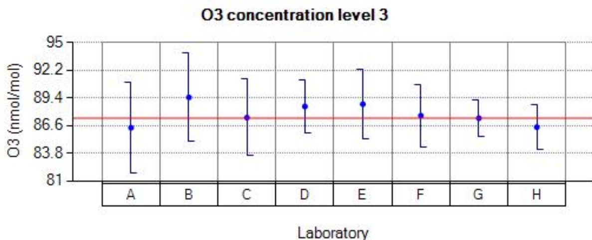
Figure 28: Reported values for O 3 run 3.
