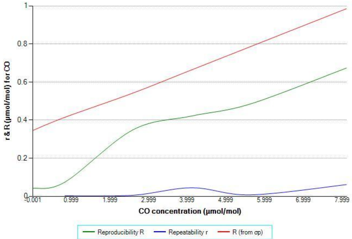
Figure 49: The R and r of CO standard measurement method as a function of concentration.
