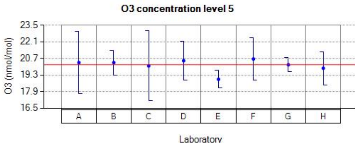
Figure 30: Reported values for O 3 run 5.
