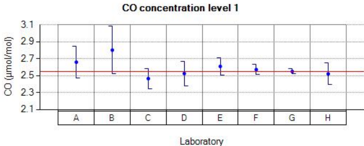
Figure 20: Reported values for CO run 1.
