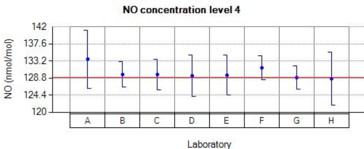
Figure 35: Reported values for NO run 4.
