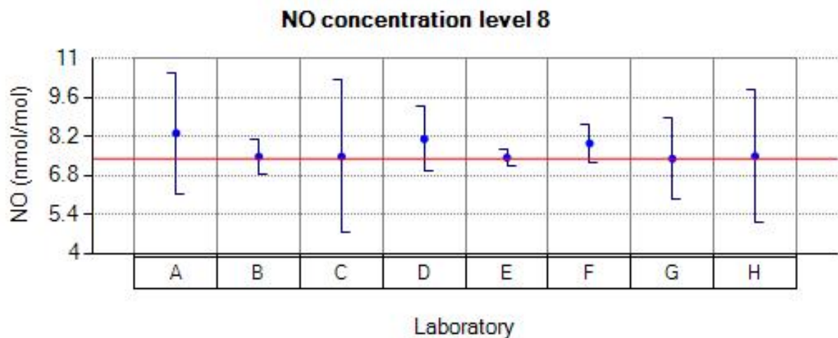
Figure 39: Reported values for NO run 8.
