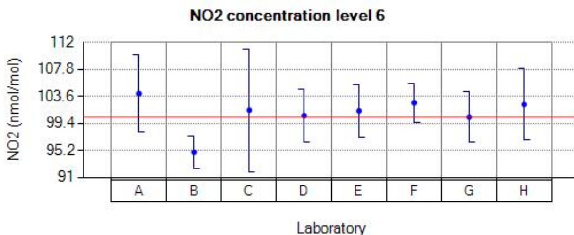
Figure 45: Reported values for NO 2 run 6.
