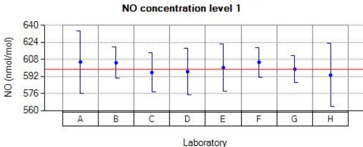
Figure 32: Reported values for NO run 1.
