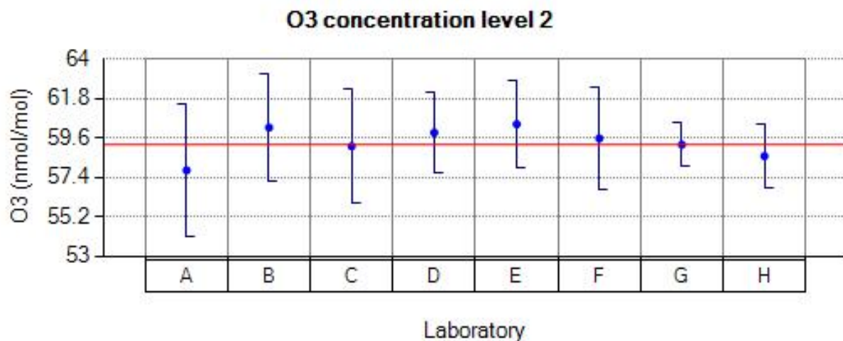
Figure 27: Reported values for O 3 run 2.
