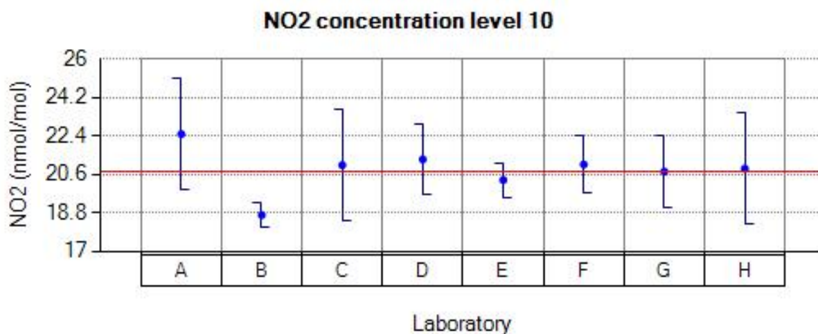
Figure 47: Reported values for NO 2 run 10.
