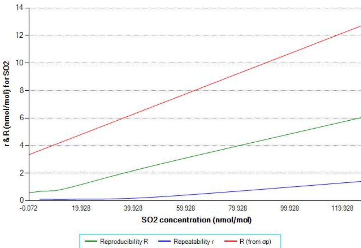
Figure 48: The R and r of SO 2 standard measurement method as a function of concentration.
