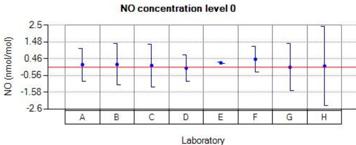
Figure 31: Reported values for NO run 0.
