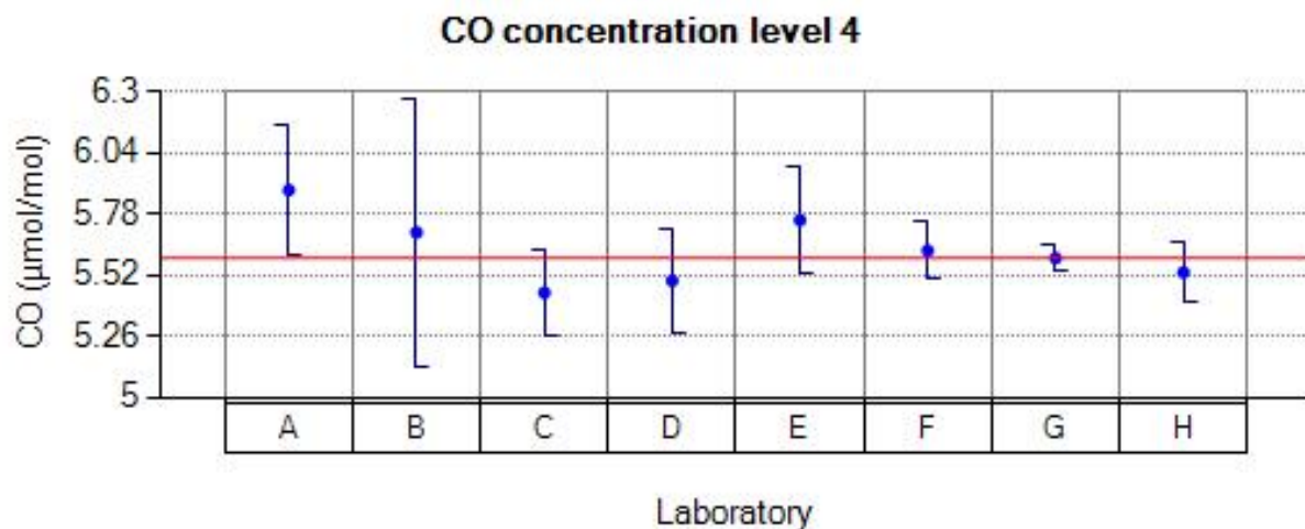
Figure 23: Reported values for CO run 4.
