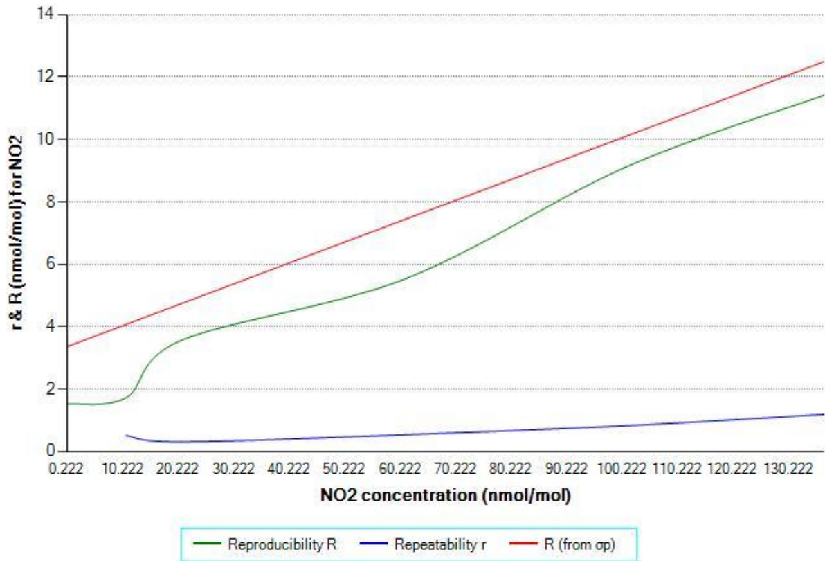
Figure 52: The R and r of NO 2 standard measurement method as a function of concentration.
