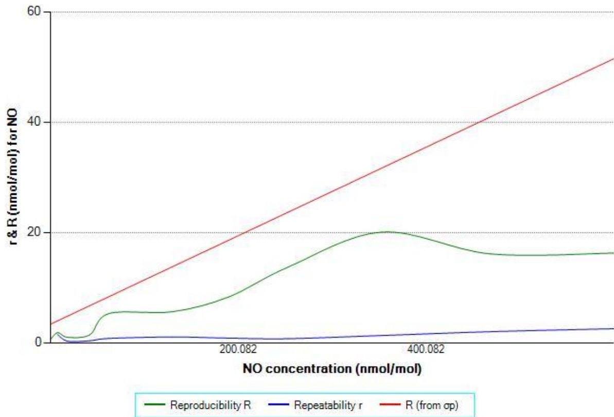
Figure 51: The R and r of NO standard measurement method as a function of concentration.
