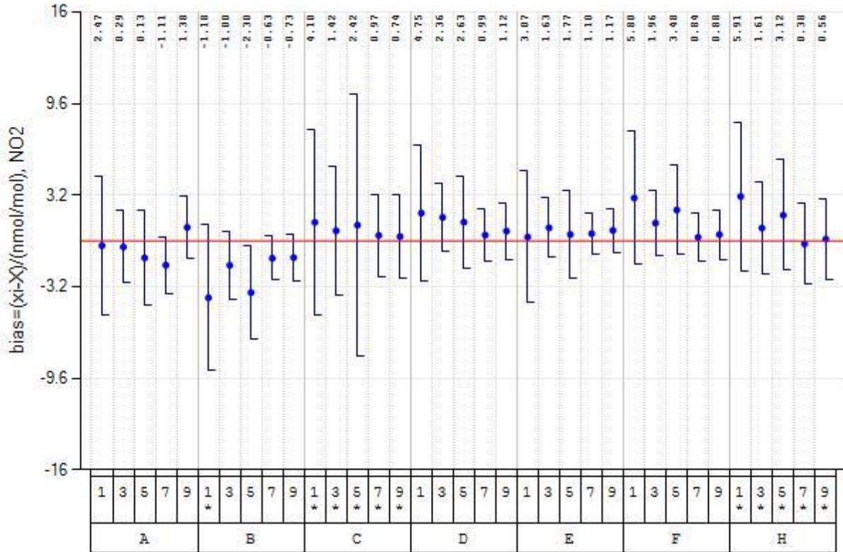
Figure 11: Bias of participant's NO 2 measurements for run numbers 1, 3, 5, 7 and 9 Within these test gas mixtures there is no gas phase titration to produce NO 2 (see Table 3). For each evaluation the run number together with the participants rounded run average (nmol/mol) is given.
