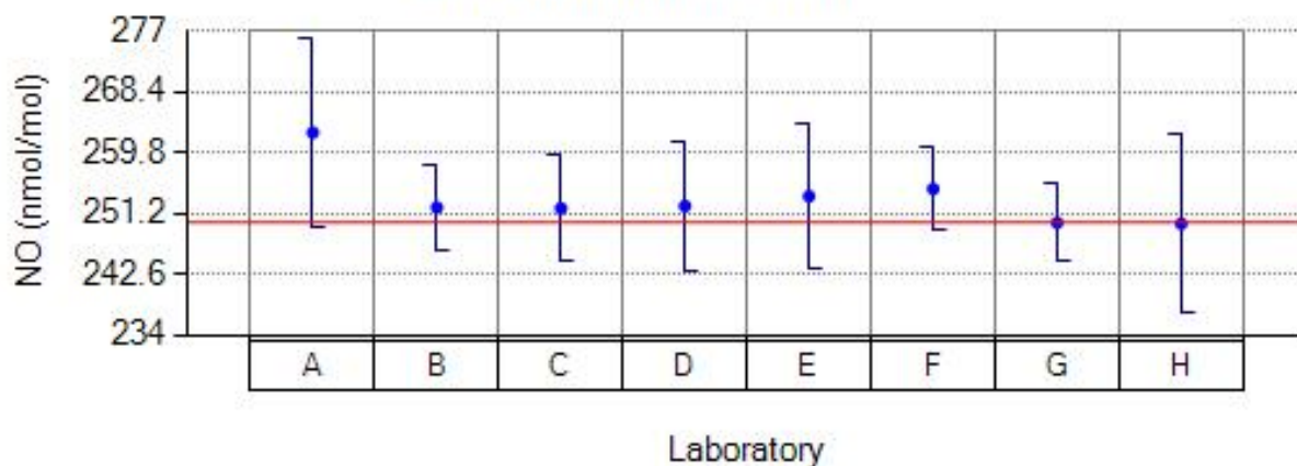
Figure 37: Reported values for NO run 6.
