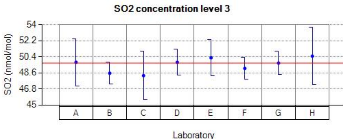
Figure 16: Reported values for SO 2 run 3.
