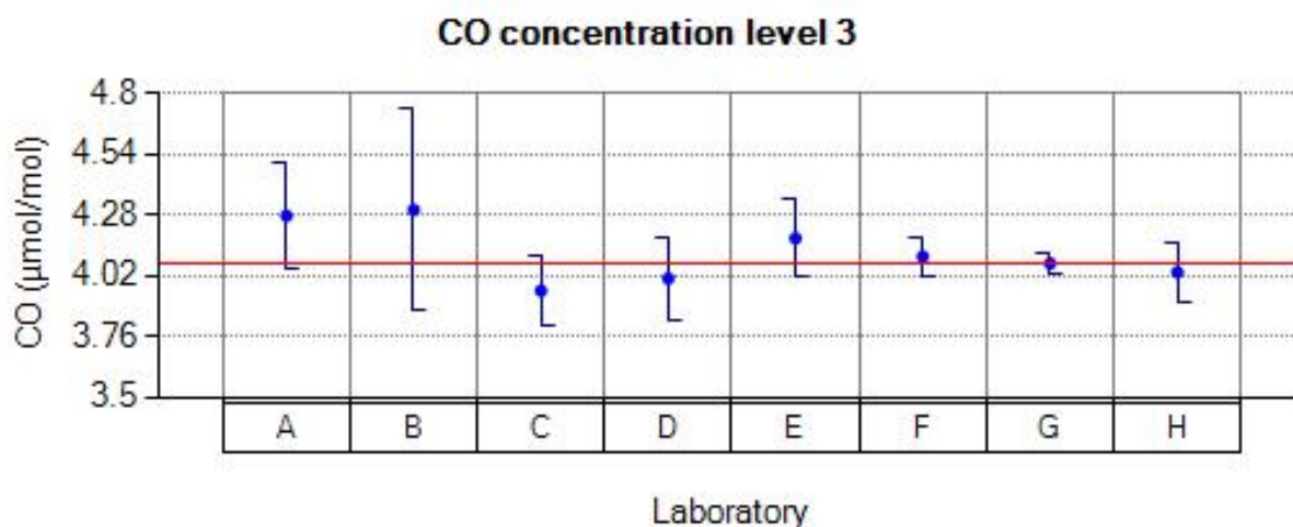
Figure 22: Reported values for CO run 3.
