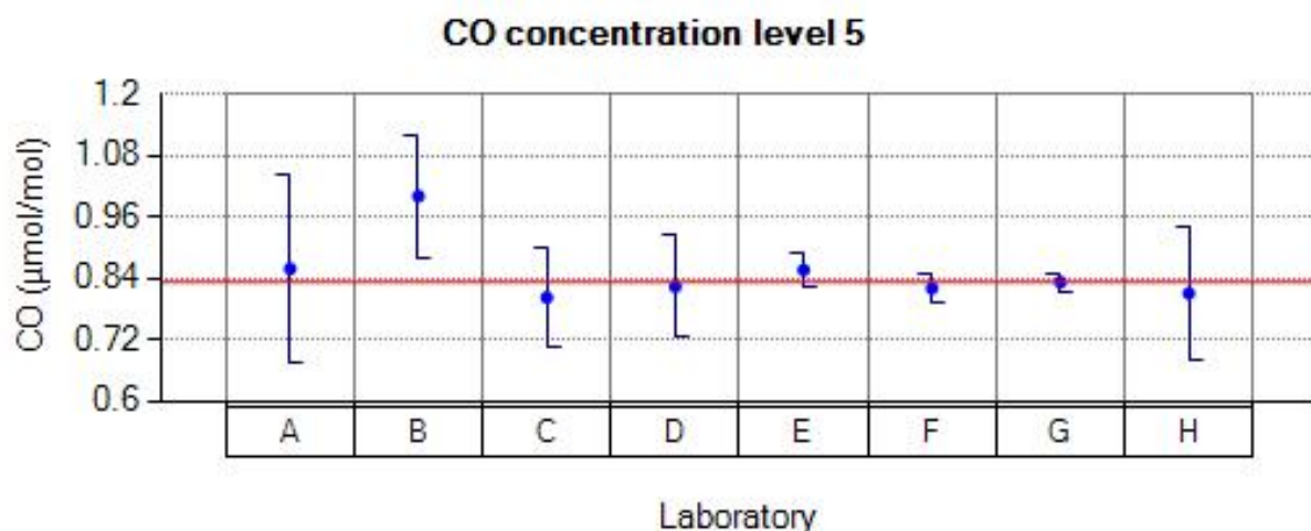
Figure 24: Reported values for CO run 5.
