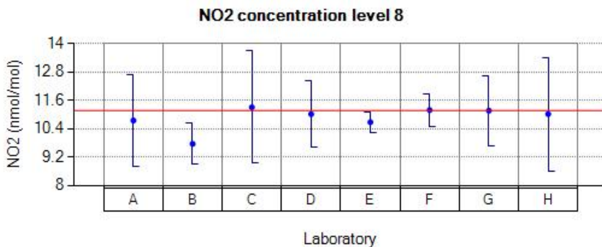
Figure 46: Reported values for NO 2 run 8.
