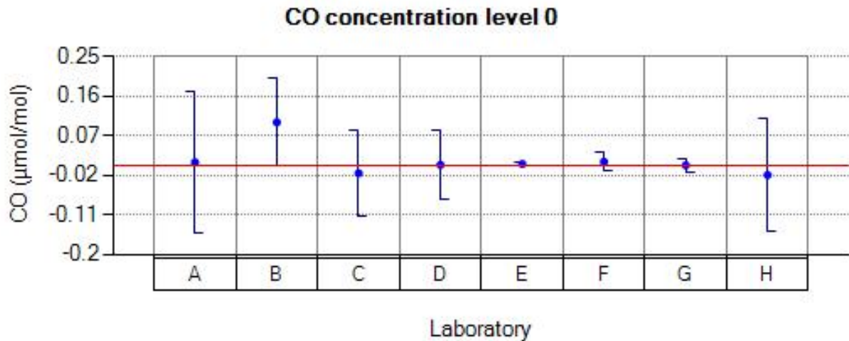
Figure 19: Reported values for CO run 0.
