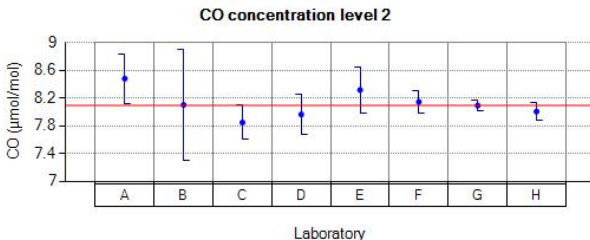
Figure 21: Reported values for CO run 2.
