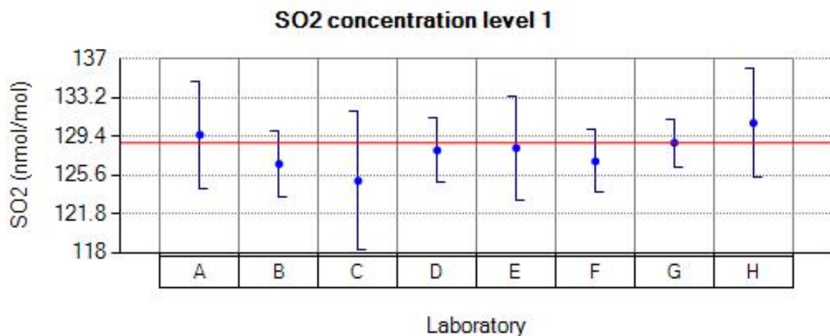
Figure 14: Reported values for SO 2 run 1.
