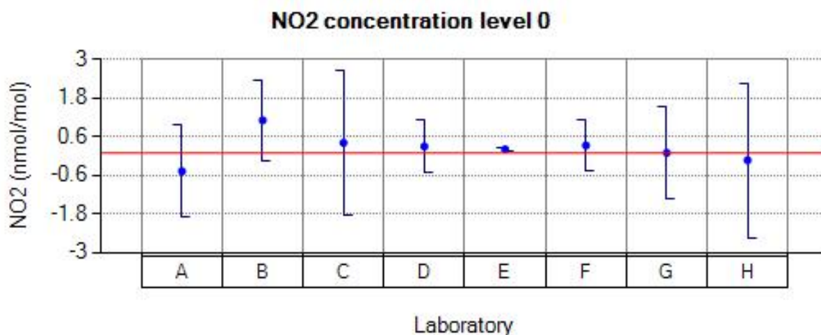
Figure 42: Reported values for NO 2 run 0.
