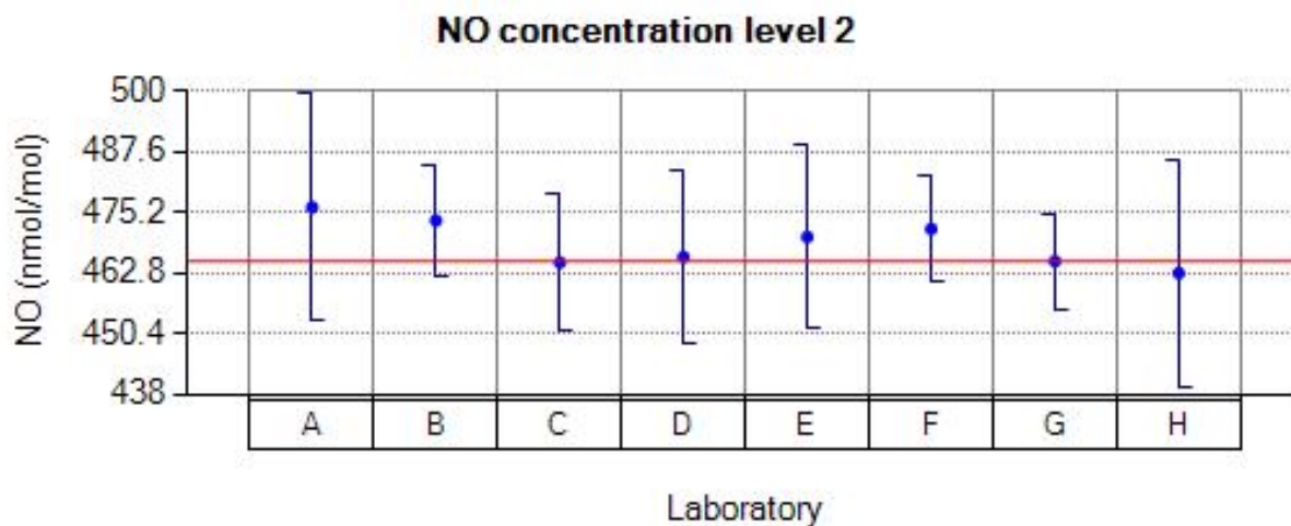
Figure 33: Reported values for NO run 2.
