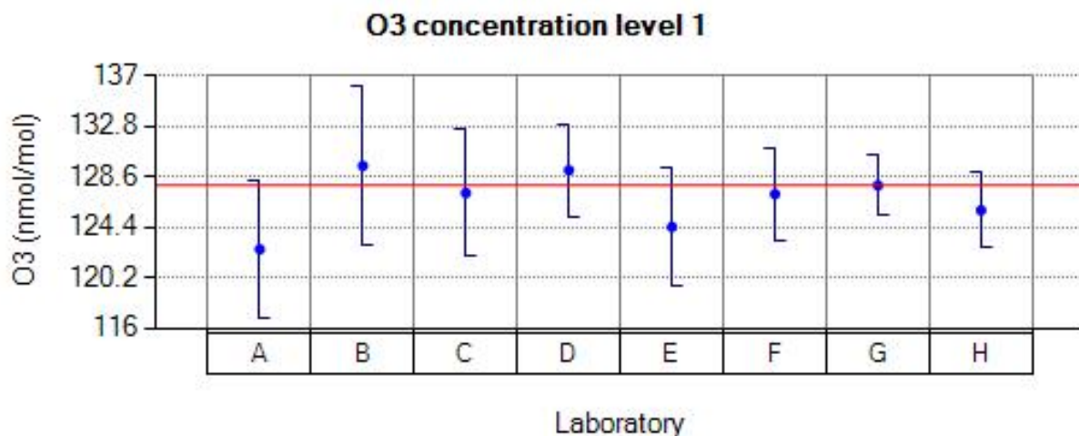
Figure 26: Reported values for O 3 run 1.
