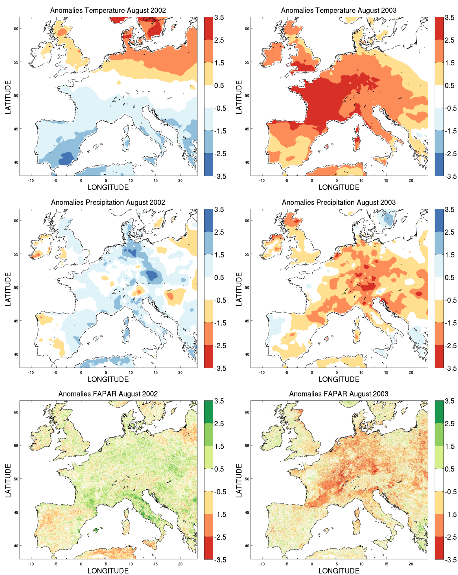
Figure 3. Monthly anomalies of surface temperature, precipitation and FAPAR for the two contrasting wet and dry periods of August 2002 ( left ), and August 2003 ( right ). Anomalies of FAPAR and surface temperature are normalized using Z-scores, i.e. , the departure from the climatological mean is divided by the standard deviation for the given month, hereafter AFAPAR and AT, respectively. Anomalies of precipitation refer to Standardized Precipitation Index (SPI)-3. Deficits and excesses in temperature are represented by shades of red and blue, respectively, while deficits and excesses in precipitation are represented by shades of blue and red. Areas of high and low photosynthetic activity are shown in shades of blue and red, respectively.
