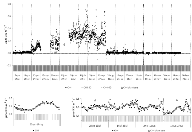
Fig. 5. Average daily variation during 2 weeks periods (with detail of CH 4 fluxes in periods with higher emissions). Data are binned by time of day and then averaged for 2 weeks periods. The standard deviations are calculated on data passing the quality test on turbulence intensity.
