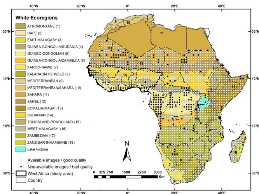
Figure 2. Availability of good quality Landsat MSS images for the 1975 reference year over sub-Saharan Africa (including our study area over West Africa) overlaid on White’s ecoregions [22].
