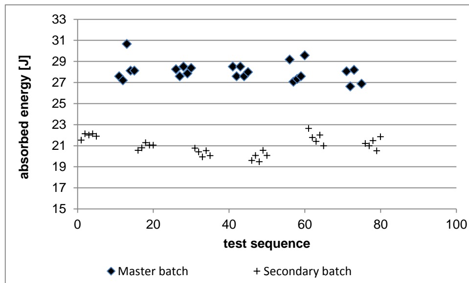
Figure 3: Absorbed energy values of 24 test pieces of ERM ® -FA013ba, compared with 30 test pieces of ERM ® -FA013bt; data are displayed in the actual test sequence
