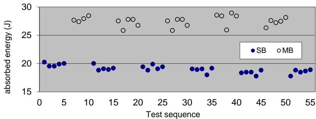
Figure 3: Absorbed energy values of 25 test pieces of ERM ® -FA013ba, compared with 30 test pieces of ERM ® -FA013bs; data are displayed in the actual test sequence
