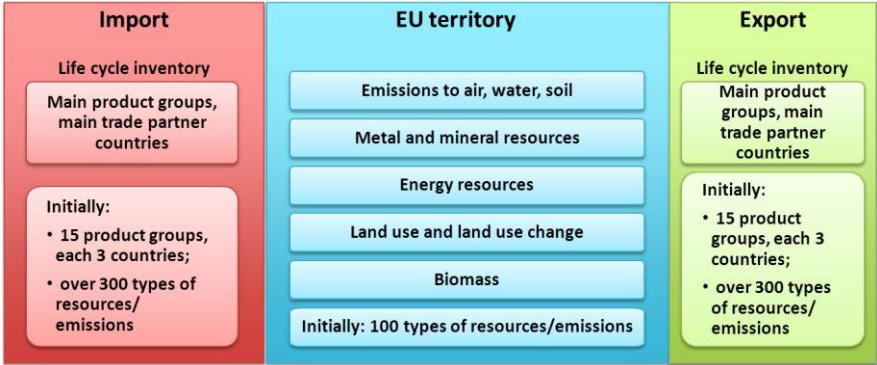
Figure 10. Coverage of the resources and emission in the total inventory and impacts (European Commission, 2012b)
