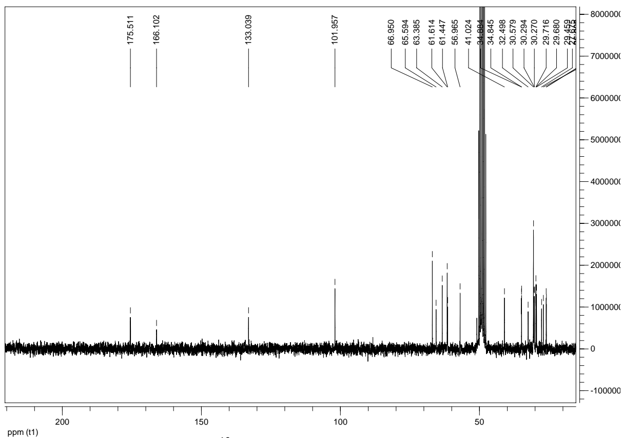
Fig. 6 ^{13}\text{C} NMR of B 12 (solvent: \text{CD}_3\text{OD} ).
