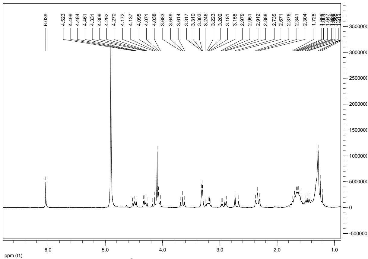
Fig. 5 ^1\text{H} NMR of B 12 (solvent: \text{CD}_3\text{OD} ).
