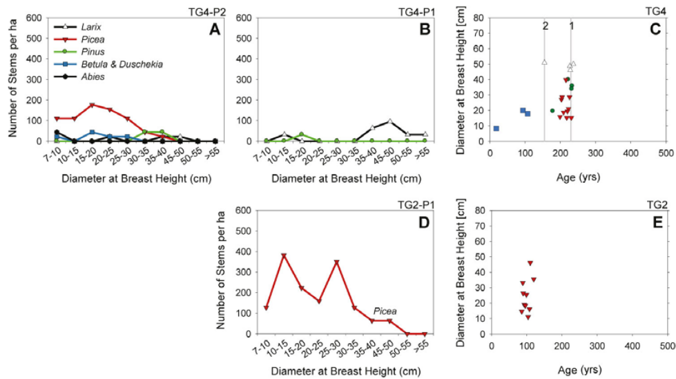
Fig. 5. Diameter at breast height of tree species growing on adjacent sites without (A) and with (B) a recent surface fire, and the relation between diameter at breast height and tree age (C), and density of trees as related to breast height diameter (D) and age (E) in a pure stand of Picea obovata which regenerated on alluvial loam. Symbols are explained in (A).
