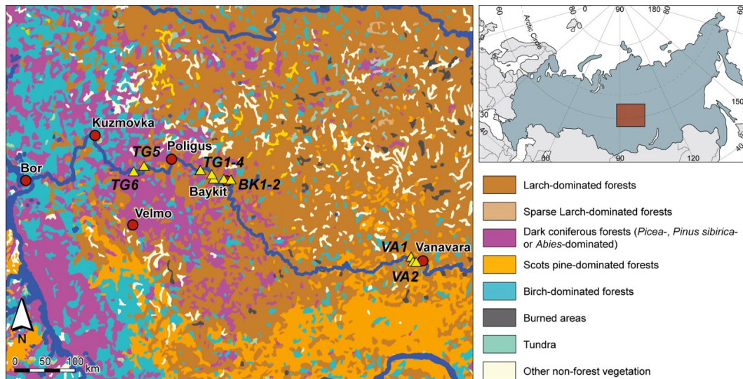
Fig. 1. Vegetation map (Isaev, 1990) and study sites at 60^{\circ} N and east of 90^{\circ} E as determined from satellite images (see site; chapter site selection). The main settlements are Bor, Kuzmovka, Velmo, Poligus, Baykit and Vanavara. The latter 4 settlements also served meteorological stations (see Table 1). The study sites are indicated as VA (Vanavara), BK (Baikit) and TG (Tunguska).
