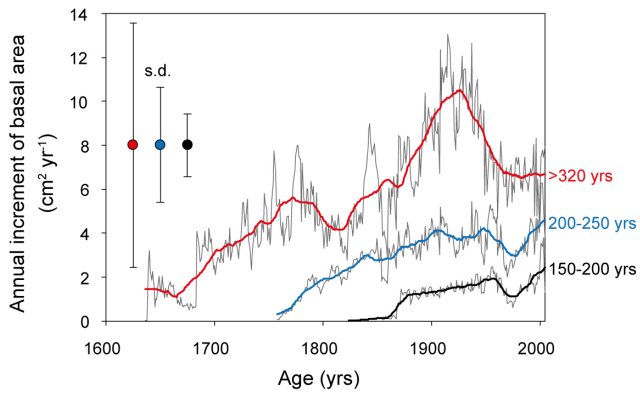
Fig. 2. Annual increment of trees as related to time before present for tree individuals older than 320 yrs ( n=9 ), of individuals between 200 and 250 yrs ( n=29 ), and of individuals between 150 and 200 yrs ( n=8 ). Depicted are averages of annual rates (thin black lines) and a smoothed line of running average over about 10 yrs, depending on the number of samples (thick red line for >320 yrs, blue line for 200 to 250 yrs and black line for 150 to 200 yrs).
