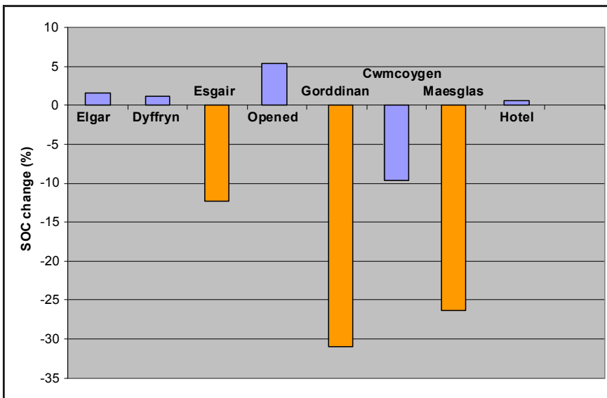
Figure 6: Total SOC change between 1978/80 and mean of 2003/05 for correctly sampled sites
