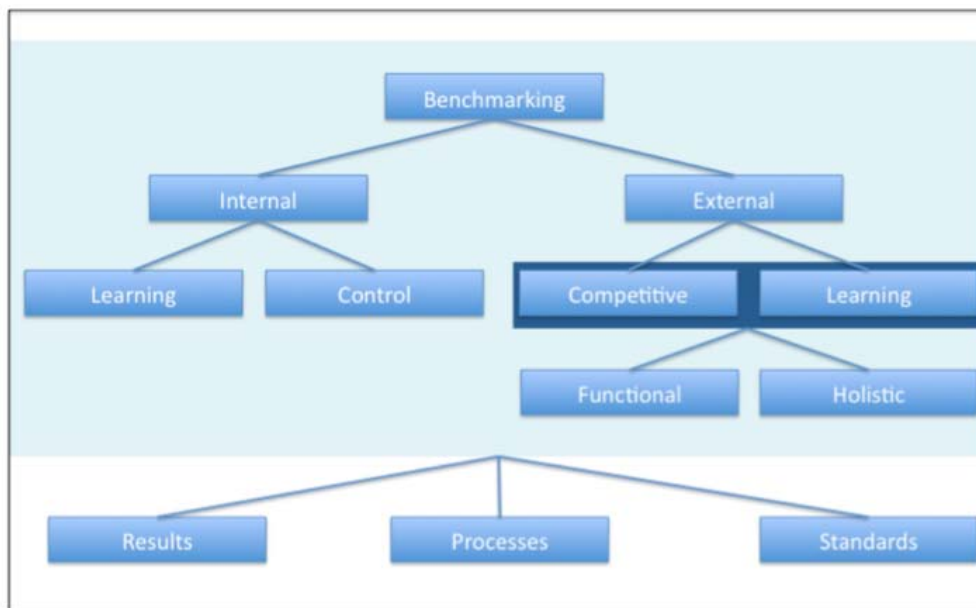
Figure 1: Benchmarking typology
