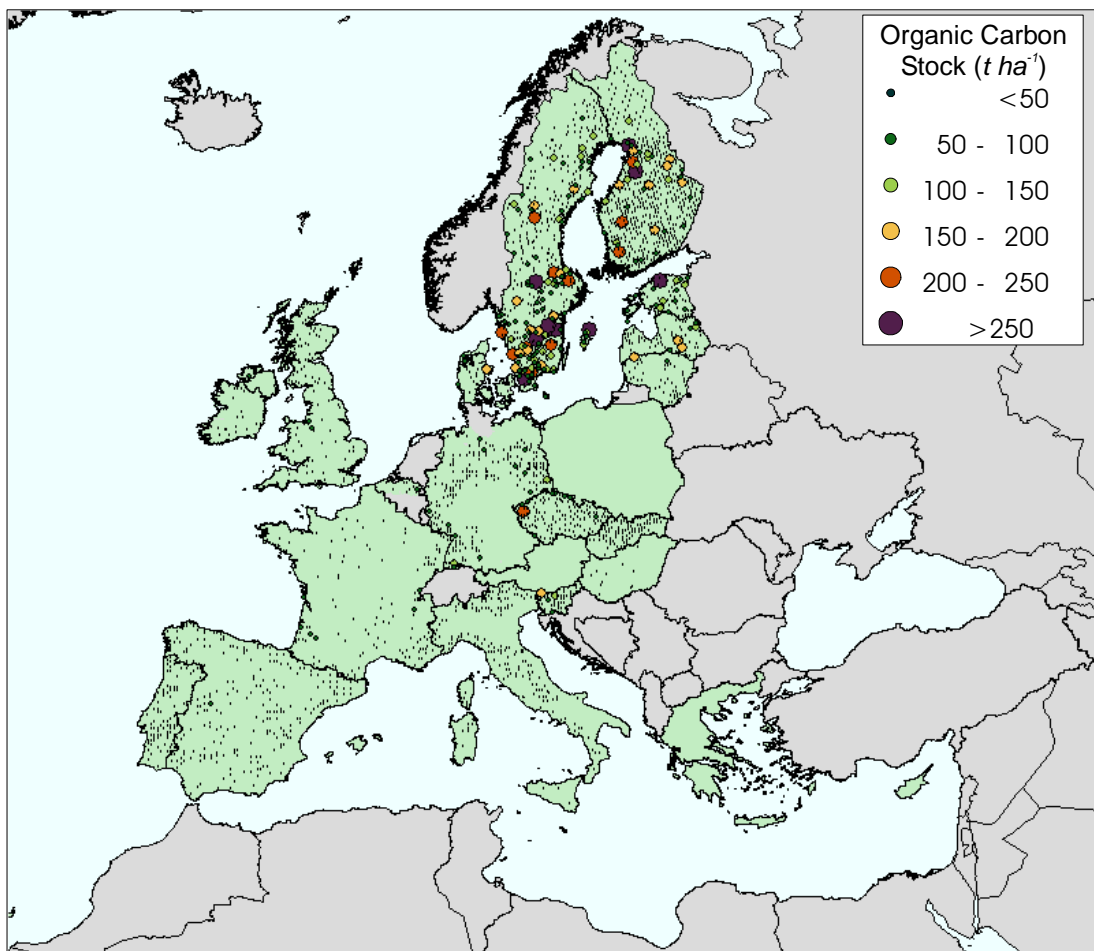
Figure 32: Organic Carbon Quantity in Organic Layer (Level 1)
