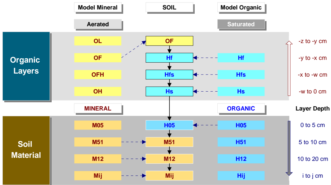
Figure 10: Schematized Arrangement of Soil Sample Layers
