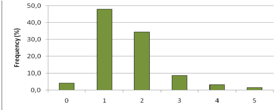
Figure 75: Frequency of Number of Qualifiers Applied for Podzols
