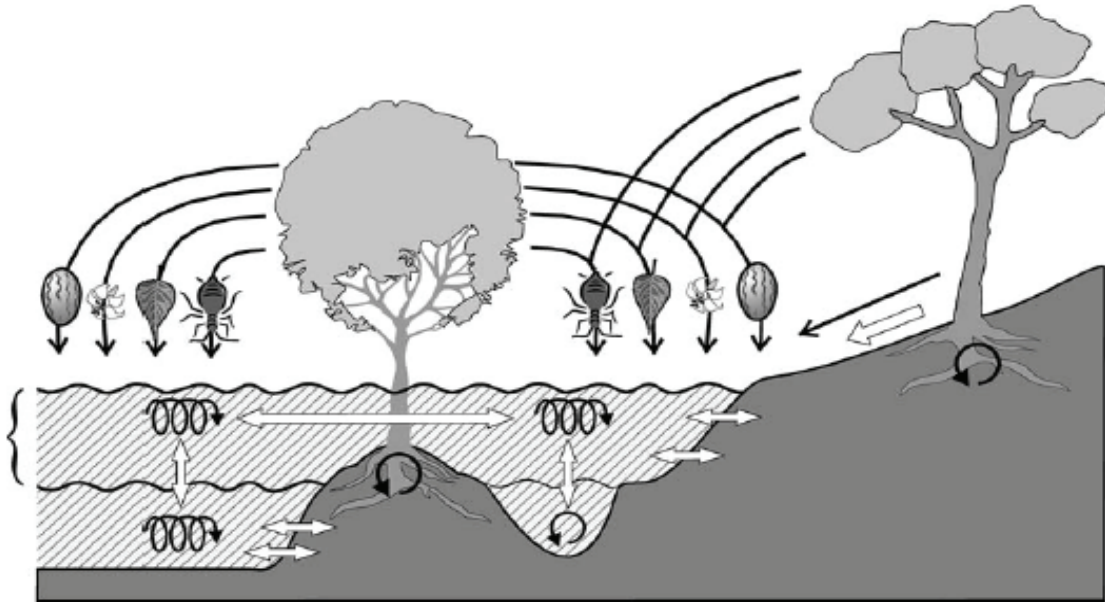
Fig. 10 Inputs, turnover, and exchange of organic matter in the stream channel (left) and a riparian wetland water body (center) at low and high water levels. Black arrows indicate organic matter inputs, white arrows indicate water exchange pathways, spirals indicate nutrient spiralling or downriver transport, and circular arrows indicate sites of organic matter turnover in situ. Curly brace indicates water-level fluctuations during flood events (Wantzen & Junk, 2008).
