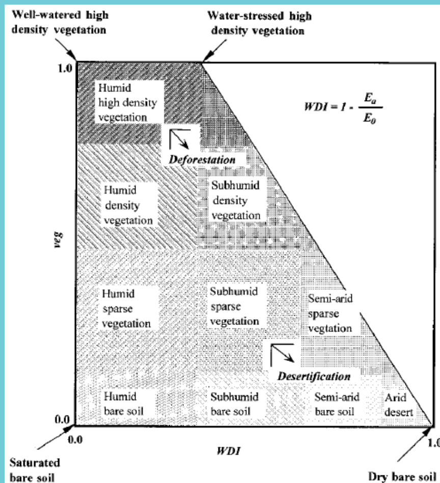
Fig. 6 A theoretical scheme showing different land use types vs WDI and vegetation fraction (veg), and the direction of desertification and deforestation vs these two indices (Wang & Takahashi, 1999).
