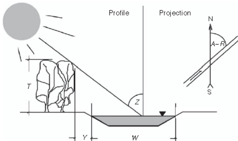
Fig. 8 Scheme to estimate optimal parameters of streamside vegetation to stream surface shade
