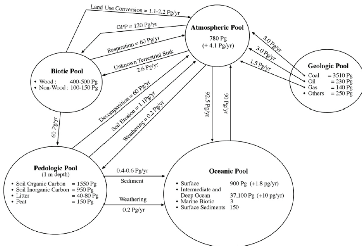
Fig. 1 Estimates of the global carbon pools and fluxes between them (Lal, 2008)
