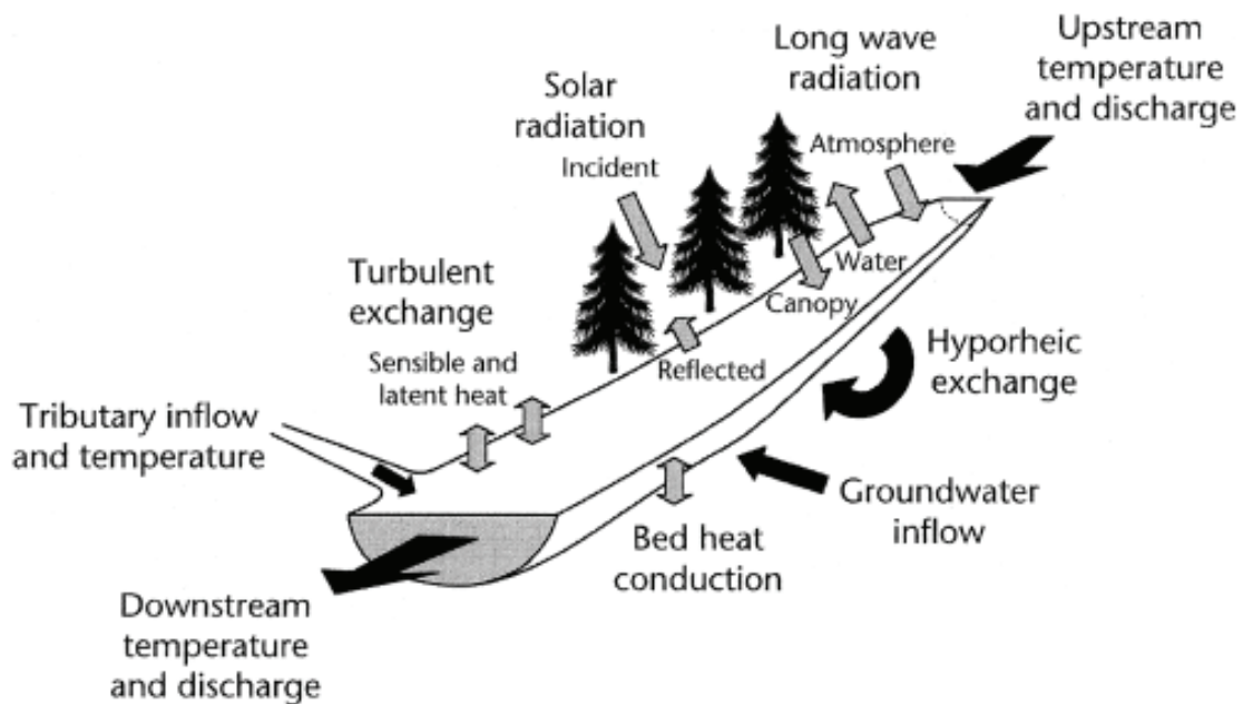
Fig. 7 Factors controlling stream temperature. Energy fluxes associated with water exchanges are shown as black arrows (Moore et al., 2005)
