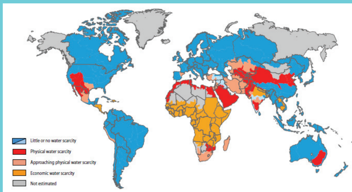
Fig. 5 Areas of physical and economic water scarcity
