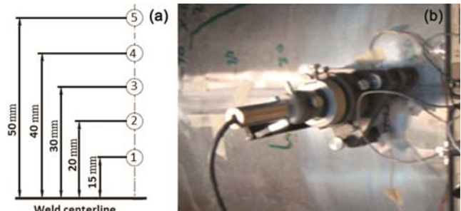
Fig. 4 — Welding residual stress measurement (a) gauge positions and (b) hole drilling machine.
