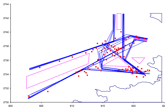
Fig. 6. Simulated places of collisions in scenario 1 (100% increase of traffic) during 800x5 years period
