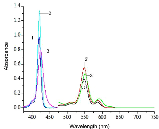
Fig. 2—UV-vis spectra of zinc porphyrins, 4a , 4b and 4c . [Curves 1, 2, and 3 are Soret bands of 4a , 4b and 4c respectively. Curves 1', 2', and 3' are Q bands of 4a , 4b and 4c respectively].
