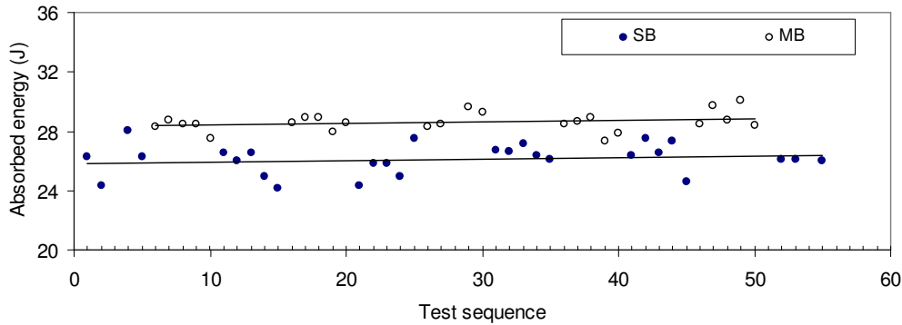
Figure 3: Absorbed energy values of the 27 test pieces of ERM®-FA013be and 24 test pieces of ERM®-FA013ba displayed in the actual test sequence.
