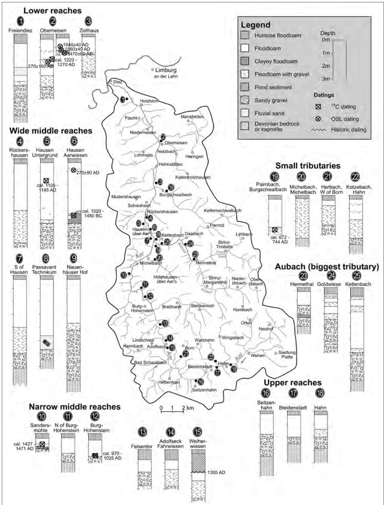
Fig. 2 Typical profiles of the Aar floodplain at 25 investigated locations which show the distribution and characteristics of the floodplain deposits. Each profile has been selected from 2 to 30 drillings and excavations (data of sites No. 7, 8, 9, 11, 16, 17, 18, 20, 22, 23, 25 by Hessisches Landesamt für Umwelt und Geologie, drilling archive; cartography: S. Böhnke).
