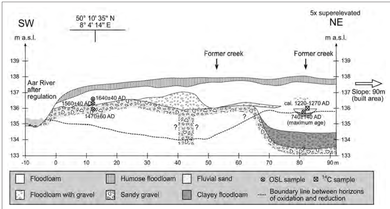
Fig. 6 Cross-section of the Aar floodplain near the village of Oberneisen (Fig. 2, No. 2)
