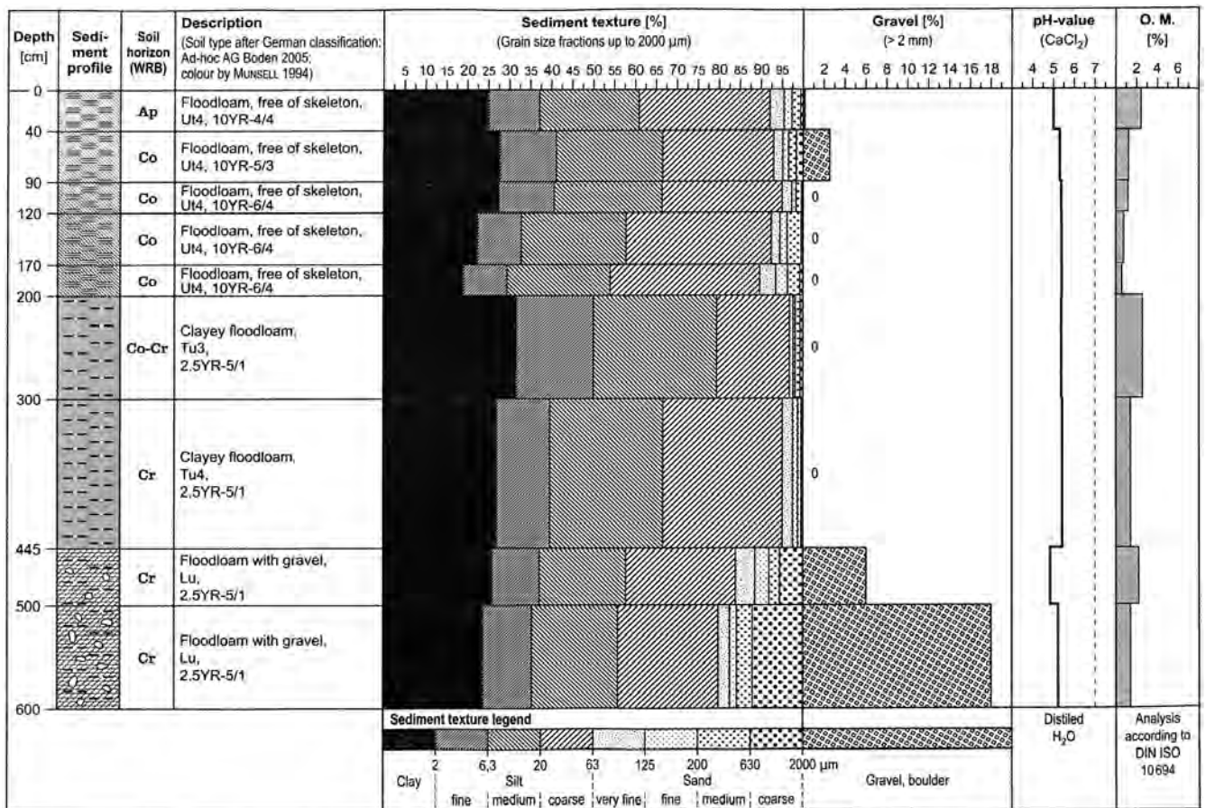
Fig. 3 A typical profile from the floodplain of the Aar River near the village of Rückershausen (50°26' N, 8°06' E; design: T. Bartsch, Mainz University)
