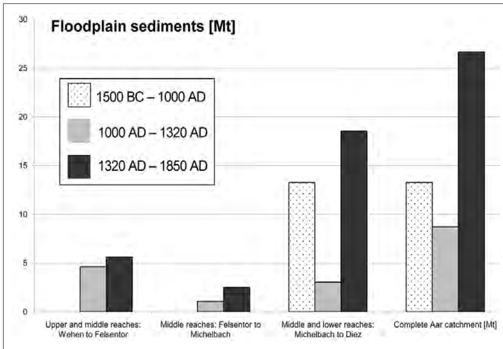
Fig. 7 Spatiotemporal quantification of floodplain sedimentation in the Aar catchment
