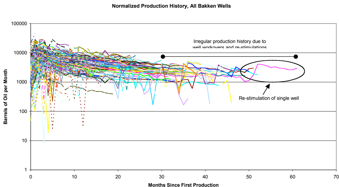
Fig. 1 Monthly Decline Curves for 225 New MT Bakken Wells Showing Re-stimulation of One Well Mid-2000 to 2005 Completions Normalized to Number of Months Since First Production Reported Monthly Production (BO/month, no matter how many days in production)
