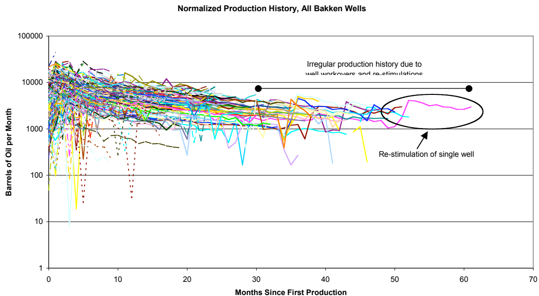
Fig. 1 Monthly Decline Curves for 225 New MT Bakken Wells Showing Re-stimulation of One Well Mid-2000 to 2005 Completions Normalized to Number of Months Since First Production
