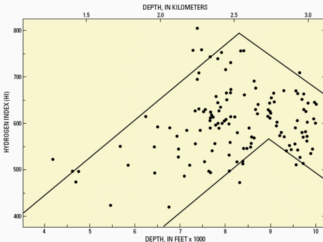
Figure 7. Plot of the ROCK-EVAL hydrogen index versus burial depth in feet and kilometers, for immature upper and lower Bakken Formation shales, Williston Basin, and for Bakken shales which have just commenced HC generation where total shale thickness is 17 ft (5.3 m) or greater.
