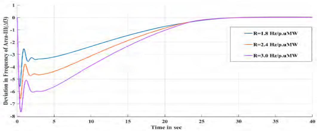
(c) Control Area-III
