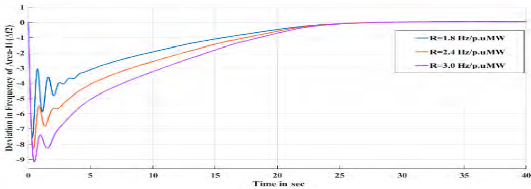
(b) Control Area-II
