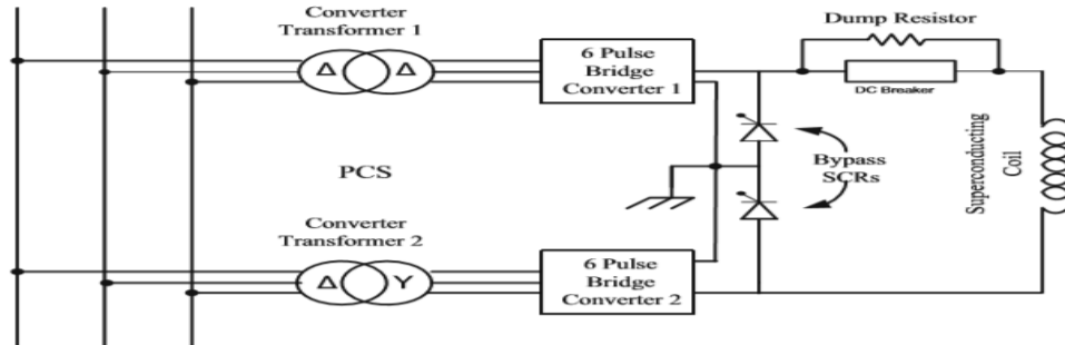
Figure 3: Configuration of SMES in power system
