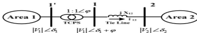
Figure 1: Schematic representation of TCPS in series with tie line for two-area control network
