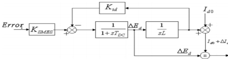
Figure 4: Block diagram representation of SMES unit
