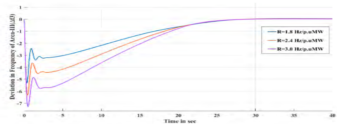
(c) Control Area-III
