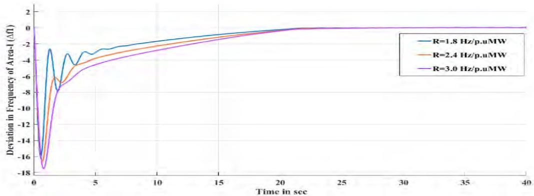
(a) Control Area-I
