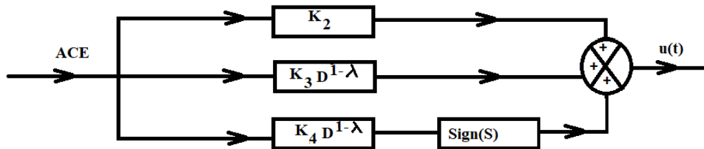
Figure 5: FOSMC representation for global rule enforcement
