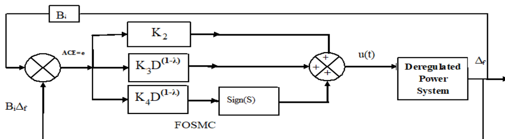
Figure 6: Block diagram layout of FOSMC control rule for DPS application
