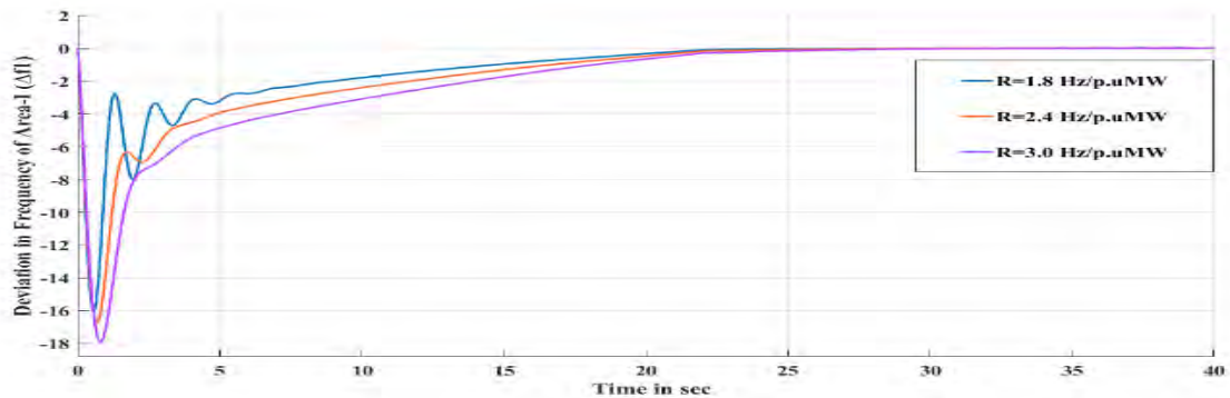
(a) Control Area-I
