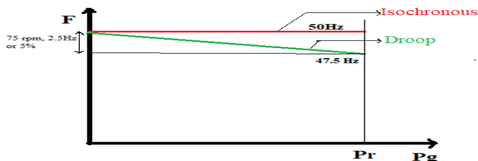
Figure 7: Illustrates Isochronous governor and Droop governor
