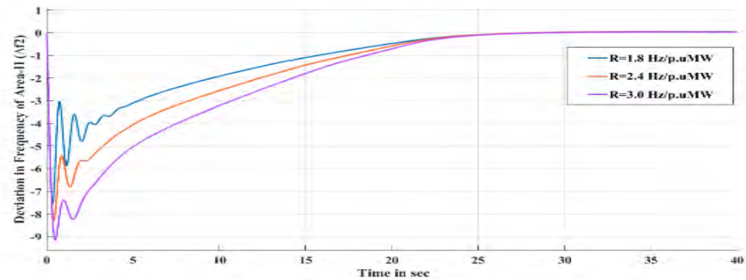
(b) Control Area-II
