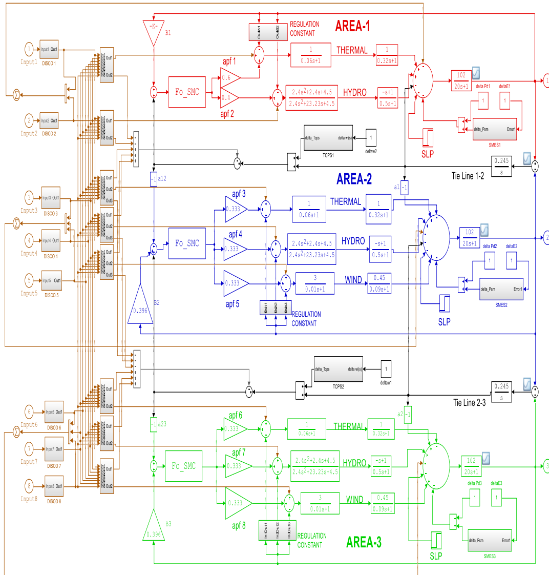
Figure 8: Simulation model of the three-area LFC multi-unit deregulated power system including combination of FOSMC and TCPS-SMES
