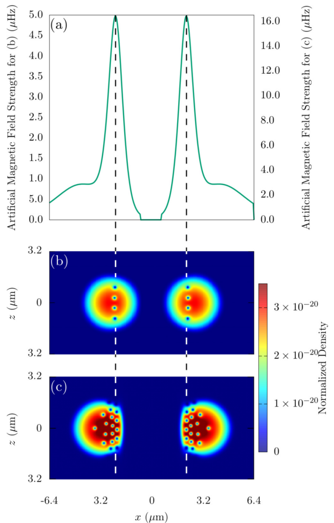
FIG. 5. (a) The magnetic field profile along the x direction for the fundamental HE_{11} mode with circular polarization outside a fibre of 200 nm radius. Note that for this mode and polarization the whole system is azimuthally symmetric. For weak fields [see (b)] this leads to a small number of vortices that align along the line at which the magnetic field is maximal and for larger fields [see (c)] more vortex rings appear that form the beginning of an Abrikosov lattice. The optical fiber field and wave-function density have been normalized and are for a nanofiber of 200 nm in diameter with blue-detuned light of 700 nm and a ^{87}\text{Rb} BEC respectively.
