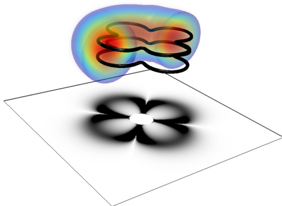
FIG. 4. Vortex configuration for the HE_{21} mode with linear polarization along the \hat{y} direction. The vortex distributions have been found via an isosurface on the Sobel filtered wave function density for a ^{87}\text{Rb} BEC and the optical fiber fields are for a nanofiber of 400 nm in diameter for the bottom image with red-detuned light of 980 nm. The magnetic field profile is similar to the one shown in Fig. 2(f), and has been calculated for a nanofiber of 400 nm radius with red-detuned light of 980 nm.
