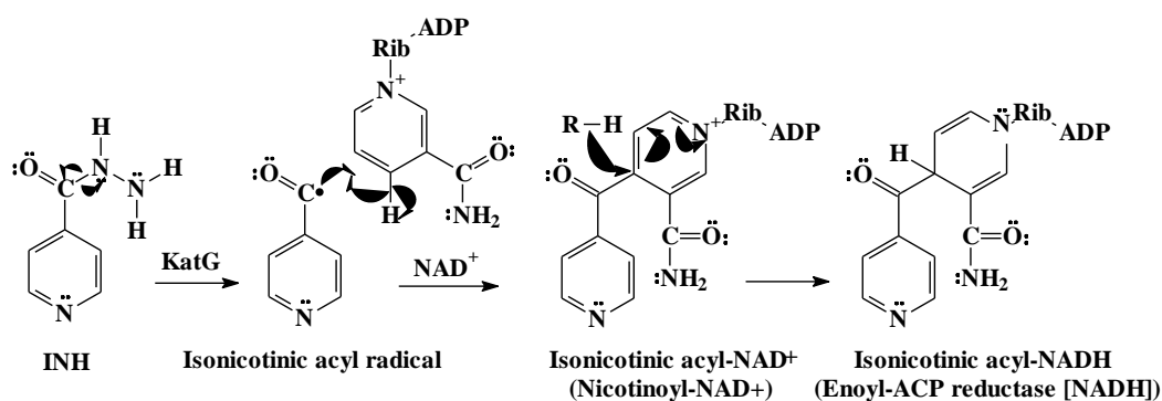
Figure 6. Mechanism of action of INH as antituberculosis (Wikipedia, 2019)
