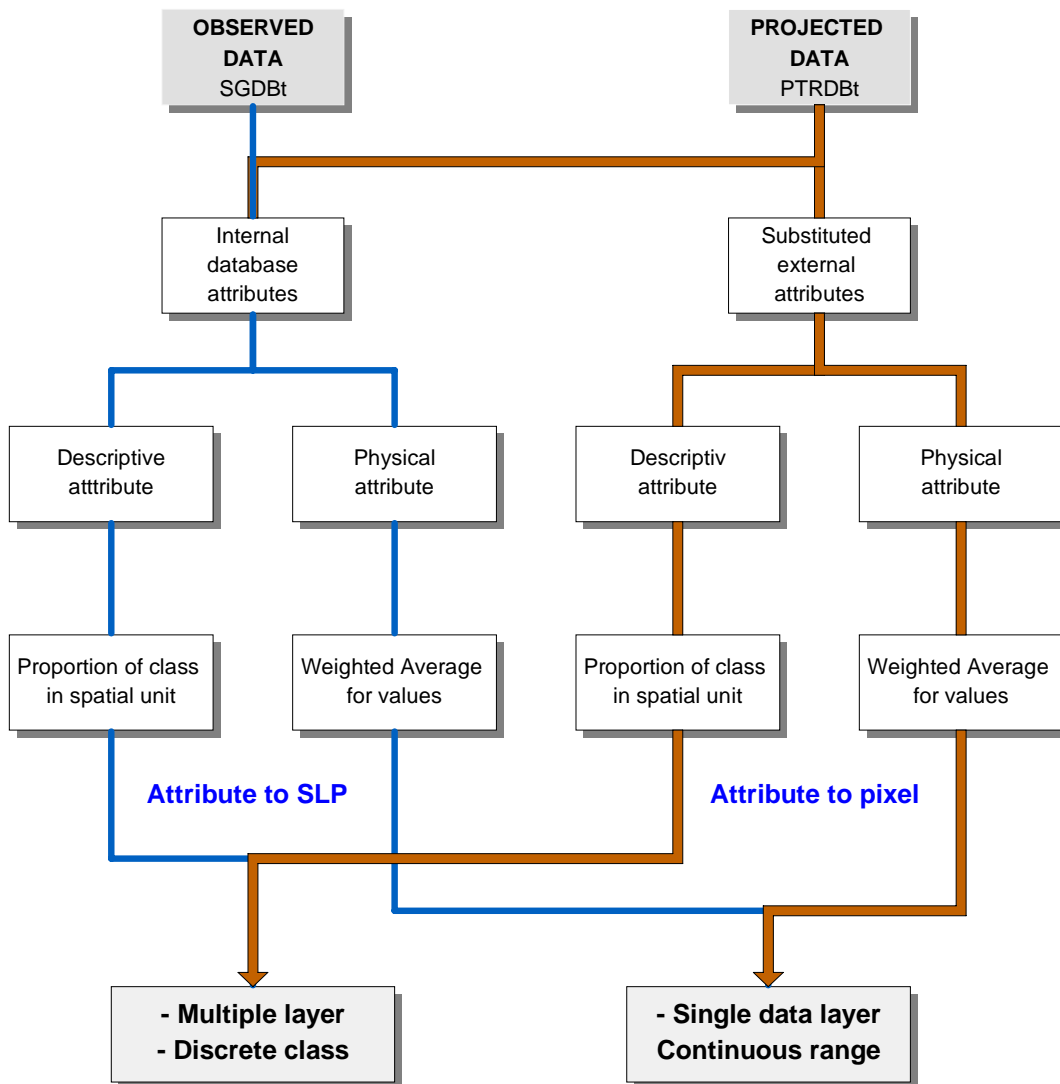
Figure 5: Output Classes of Attribute Mapping Procedure
