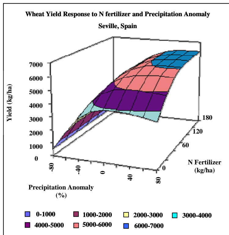
Figure 13. Wheat yield response to nitrogen fertilizer and precipitation in Sevilla, Spain
