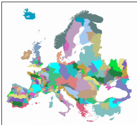
Figure 19. European basins
