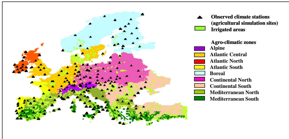
Figure 9. Spatial crop data, climate, and irrigation define agro-climatic regions
