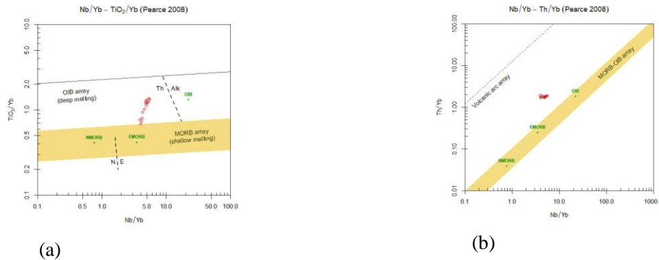
Figure 7: Determining the Tectonomagmatic environment of the upper middle Eocene volcanic rocks of Albroz in Ziaran (ZVB) using Pearce (2008) diagrams
