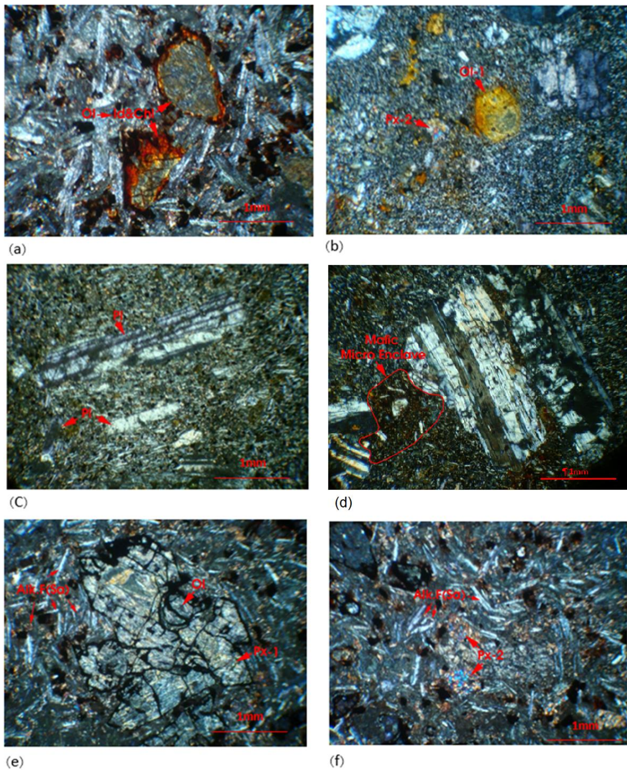
Figure 2: Microscopic images of volcanic rocks of the middle upper Eocene age in Ziaran: (a, b, c) olivine basalt, olivine (with Iddengsite edges), clinopyroxene (Cpx), titaniaaugite (Ti, Aug), plagioclase (Pl) (andesine), dark minerals (plane-polarized light, opq), (d, e, f) andesite, plagioclase (Pl) (andesine), olivine (Olv), pyroxene (Px) (plane-polarized light)
