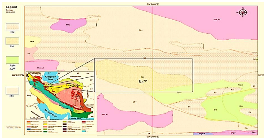
Figure 1: The location of andesite-basaltic rocks of middle Eocene age in the Central Alborz and E6ap Alamut area in the major structural-sedimentary zones of Iran (Geological Survey of Iran).
