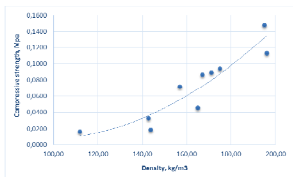
Fig.3. Compressive strength/density graph
