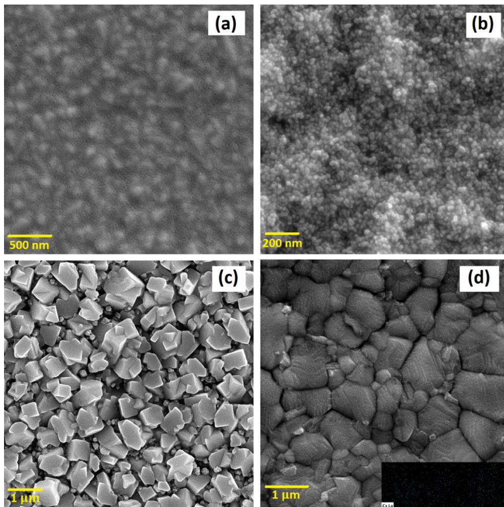
Figure 5. FESEM top views of the subsequent layers making PSC devices: (a) compact TiO 2 , (b) mesoporous TiO 2 , (c) MAPbI 3 perovskite and (d) \text{Cs}_{0.05}(\text{MA}_{0.17}\text{FA}_{0.83})_{0.95}\text{Pb}(\text{Br}_{0.17}\text{I}_{0.83})_3 perovskite, the inset shows EDS mapping of Cs.
