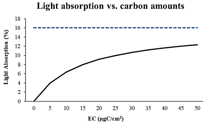
Fig. 2. Impact of particulate elemental carbon amounts on the light absorption.
