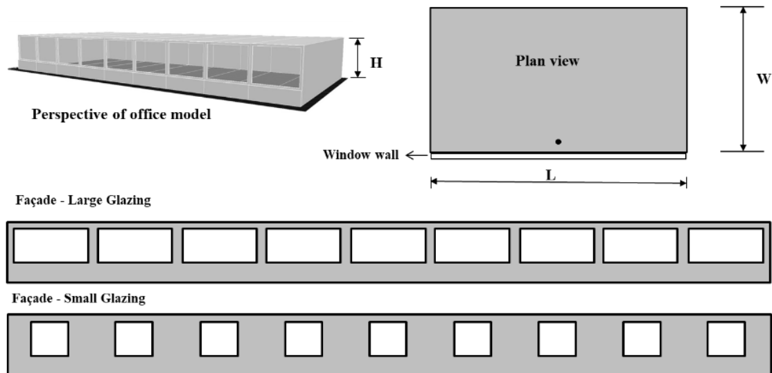
Fig. 1. The open-plan office model and glazing sizes studied.
