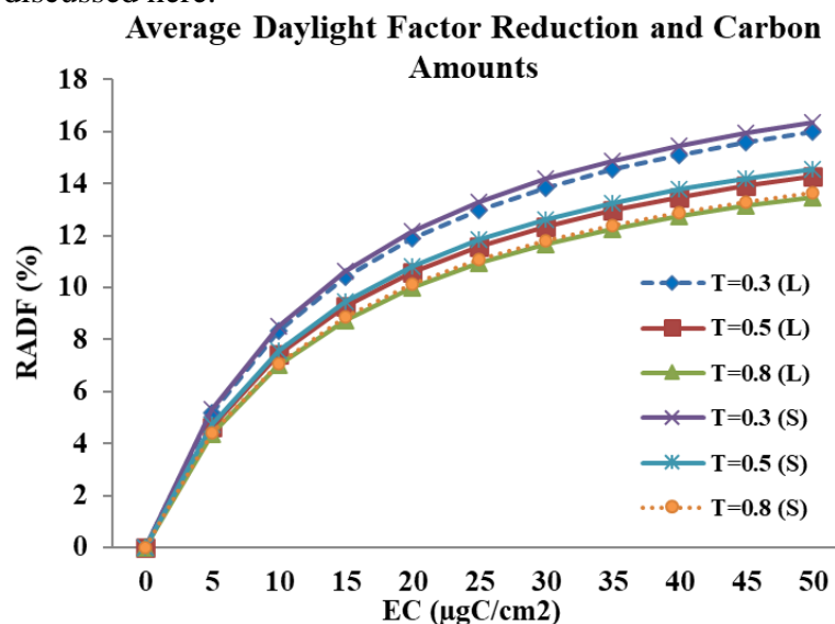
Fig. 10. The relative reduction of ADF with the increasing elemental carbon amounts at external glazing surface with three typical visual transmittances (0.3, 0.5 and 0.8).
