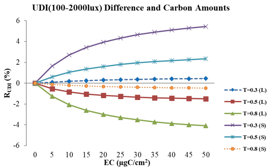
Fig. 12. The relative difference of UDI(100-2000 lux) with the increase of elemental carbon amounts of external glazing surface with three typical transmittances (0.3, 0.5 and 0.8).
