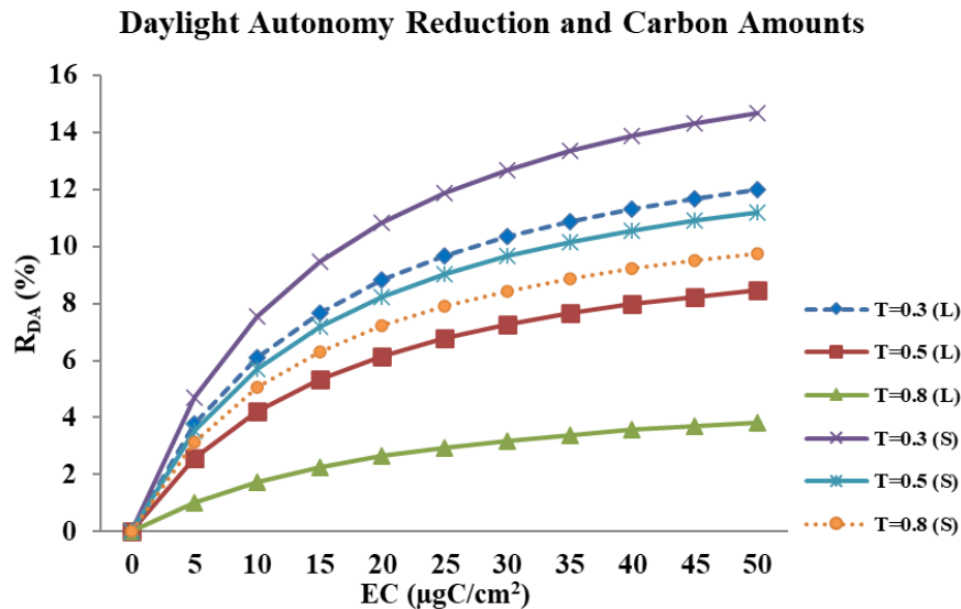
Fig. 11. The relative reduction of DA with the increase of elemental carbon amounts of external glazing surface with three typical transmittances (0.3, 0.5 and 0.8).
