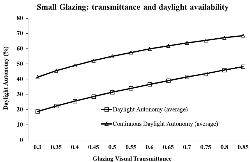
Fig. 8. The relationship between glazing visual transmittance and average daylight autonomy (small glazing area).
