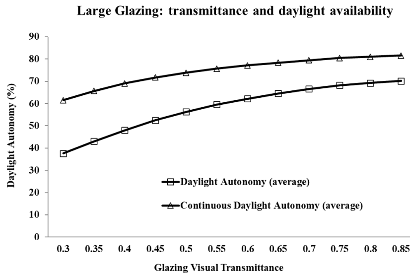
Fig. 5. The relationship between glazing visual transmittance and average daylight autonomy (large glazing area).
