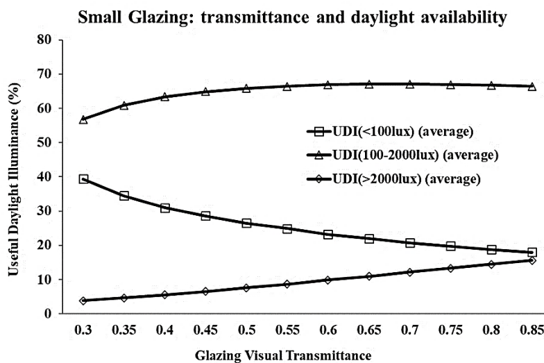
Fig. 9. The relationship between glazing visual transmittance and average useful daylight illuminance (small glazing area).
