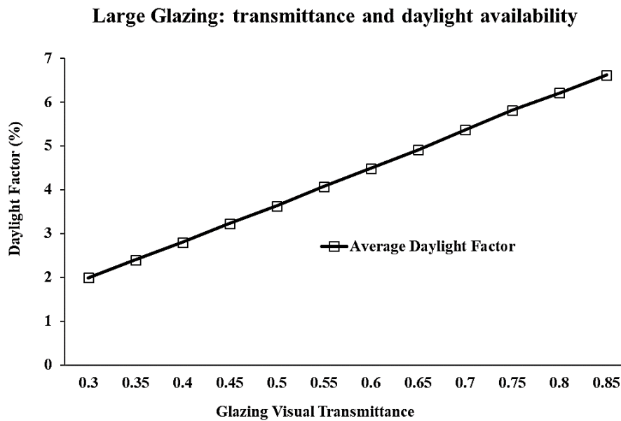
Fig. 4. The relationship between glazing visual transmittance and average daylight factor (large glazing area).
