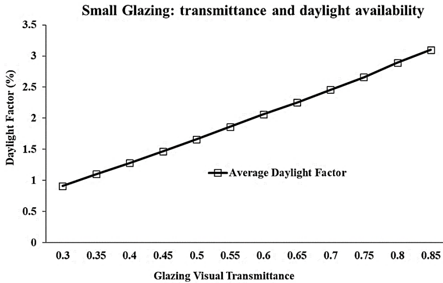
Fig. 7. The relationship between glazing visual transmittance and average daylight factor (small glazing area).
