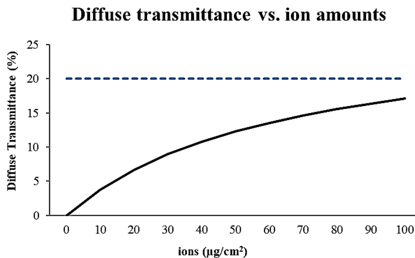
Fig. 3. Impact of soluble inorganic particle (ion) amounts on the diffuse transmittance.
