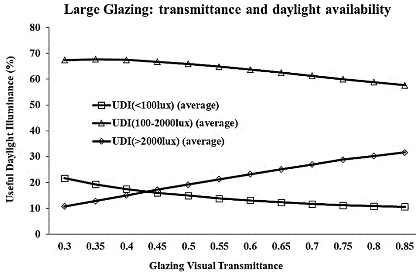
Fig. 6. The relationship between glazing visual transmittance and average useful daylight illuminance (large glazing area).
