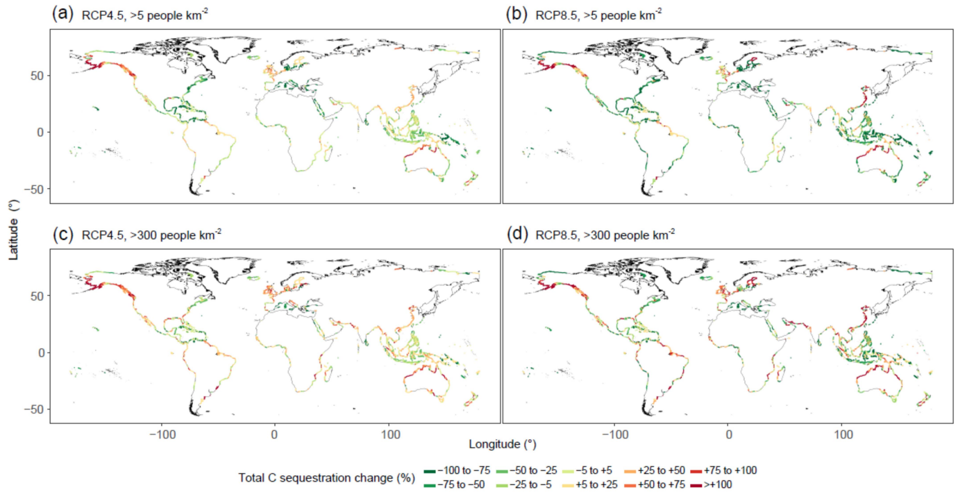
Figure 4. The projected 2100 spatial distribution of tidal wetland C sequestration changes. Relative changes in tidal wetland C sequestration are displayed for the RCP4.5 (a,c) and RCP8.5 (b,d) scenarios under two assumed human activity scenarios by Schuerch et al. [11]: inhibition of wetland inland migration in the regions with a population density (a,b) over 5 people km -2 and in the regions with a population density (c,d) of over 300 people km -2 .
