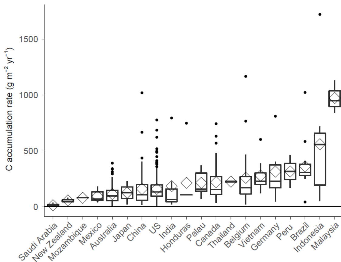
Figure 2. National C accumulation rates worldwide. The 20 countries listed here where observations are available account for 62% global tidal wetland distribution. Diamond is the mean value, the box is interquartile range, error bar is the largest and smallest value within 1.5 times interquartile range above 75% and below 25%, respectively. Black points indicate outside values.
