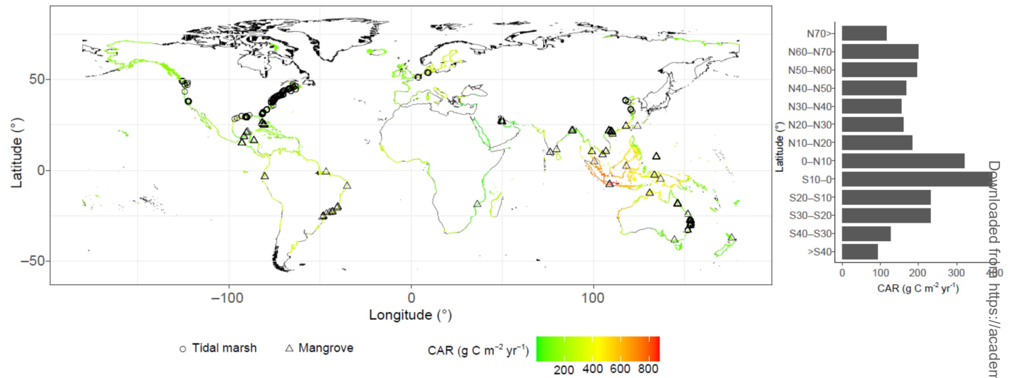
Figure 1. The spatial distribution of tidal wetlands and the observed C accumulation rate (CAR) points. The right panel indicated the arithmetic average CAR at every 10-degree bands of latitude.
