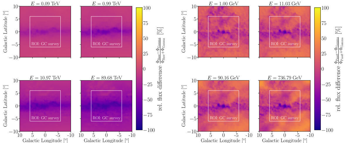
Figure 18: Left. Relative flux difference between the Gamma and Base IEMs, the square marking our ROI. Right. Same, but for Gamma and Pass8 Fermi-LAT IEMs.
