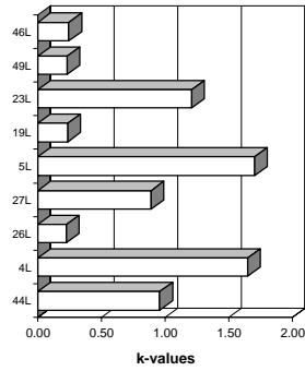
Mandel's k statistics (Sludge 1 - DEHP)
