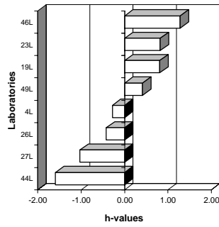
Mandel's h statistics (Soil 3 - DEHP)
