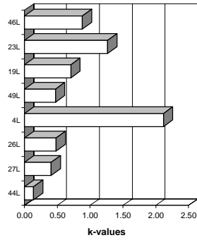
Mandel's k statistics (Soil 3 - DEHP)
