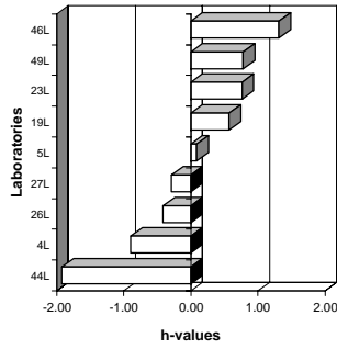
Mandel's h statistics (Sludge 1 - DEHP)
