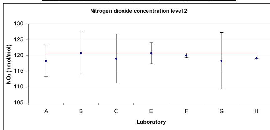
Figure 44: Reported values for NO 2 concentration level 2.
