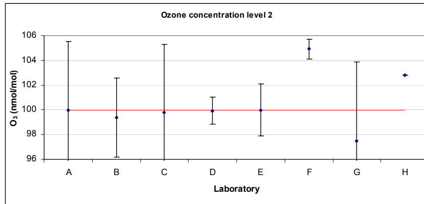
Figure 27: Reported values for O 3 concentration level 2.
