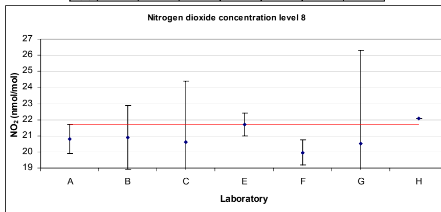
Figure 50: Reported values for NO 2 concentration level 8.
