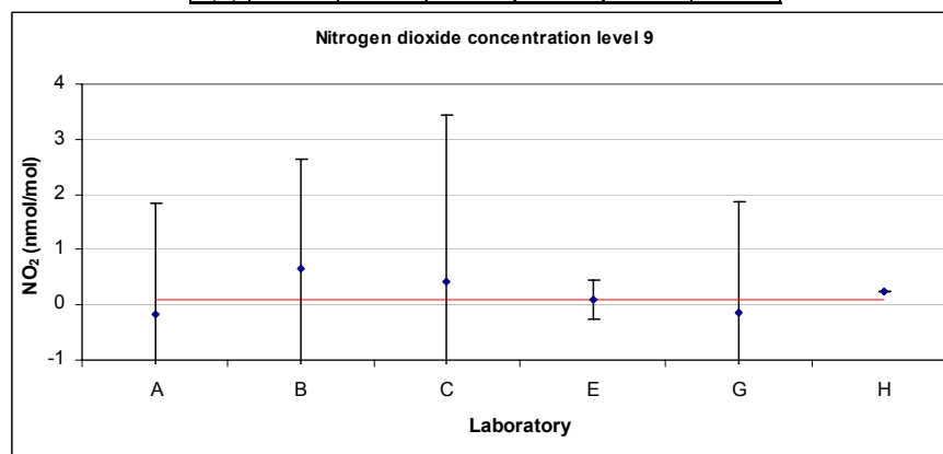
Figure 51: Reported values for NO 2 concentration level 9.
