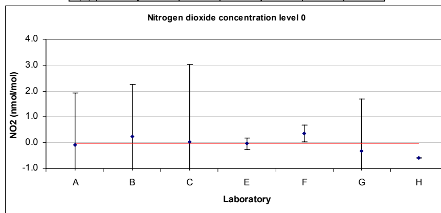
Figure 42: Reported values for NO 2 concentration level 0.
