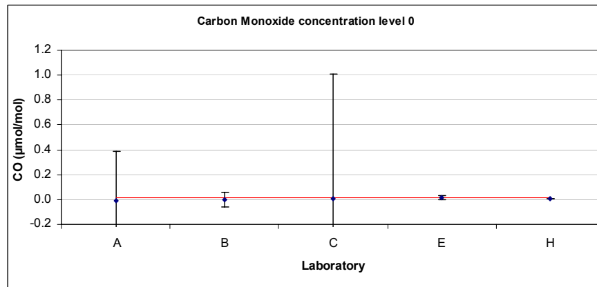
Figure 19: Reported values for CO concentration level 0.
