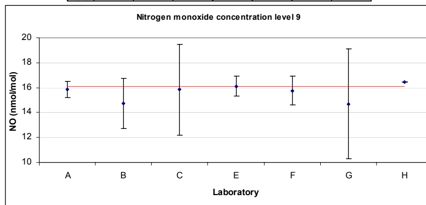
Figure 40: Reported values for NO concentration level 9.
