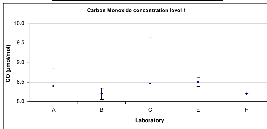
Figure 20: Reported values for CO concentration level 1.
