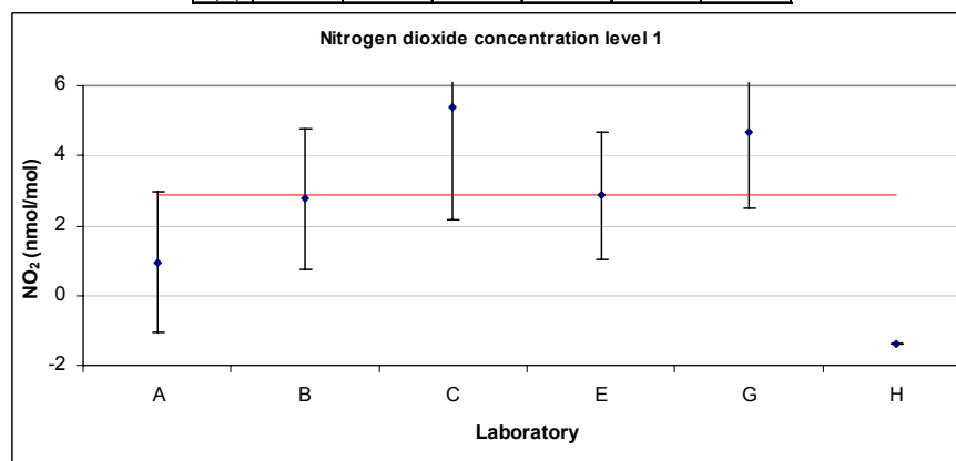
Figure 43: Reported values for NO 2 concentration level 1.
