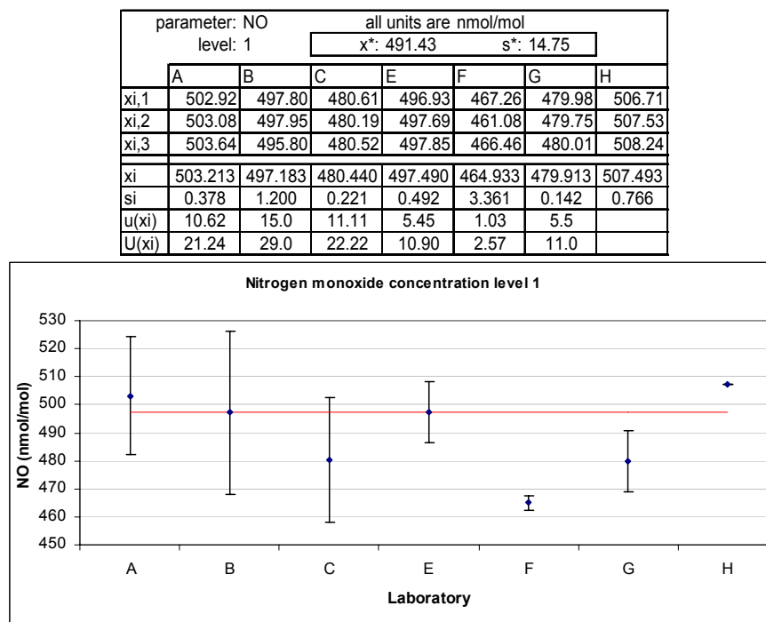
Figure 32: Reported values for NO concentration level 1.
