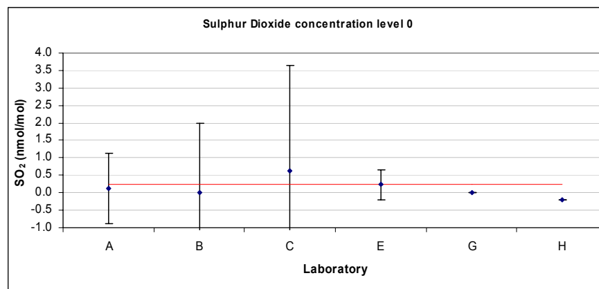
Figure 13: Reported values for SO 2 concentration level 0.
