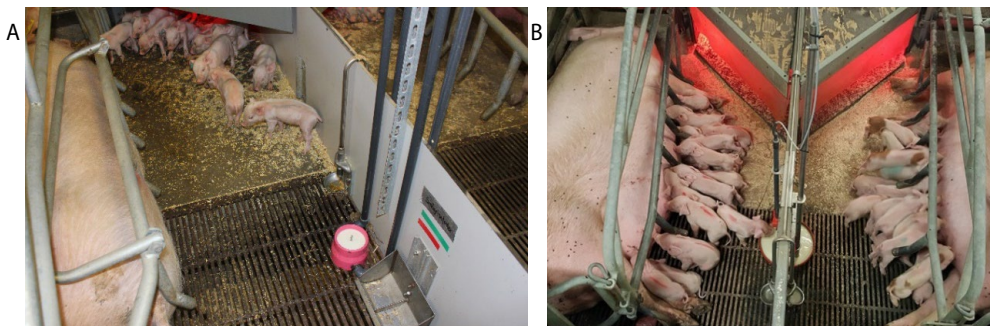
Figure 3.4. Milk cups installed in farrowing pens. (A) shows a piglet-controlled milk cup where the piglet pushes a lever with its snout to receive milk and (B) shows a self-filling larger milk bowl (photo (A) by Cecilie Kobek-Kjeldager and (B) by http://bopil.dk ).
