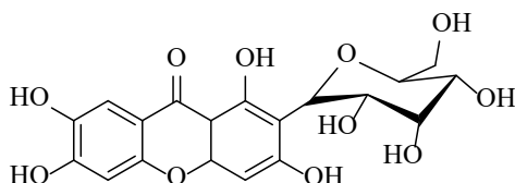
Fig. 1. Mangiferin as a biologically active representative of xanthenes
