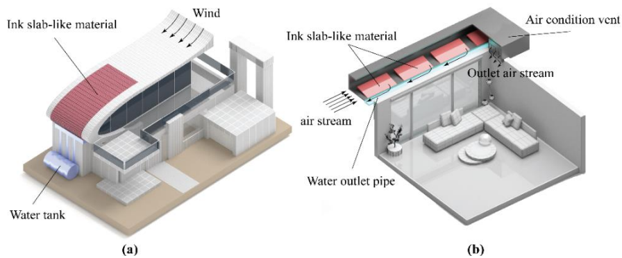
Fig. 3 (a) Exterior roof platform made of ink slab-like materials, (b) interior ink slab-like material usage in air condition vent
