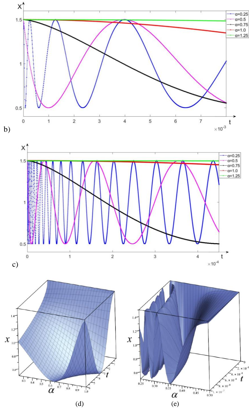
Fig. 2 Frequency property of a fractal oscillator at the initial stage for different values of \alpha . (a) \omega=1 ; (b) \omega=100 ; (c) \omega=1000 ; three-dimensional illustrations for \omega=1 (d) and \omega=100 (e)
