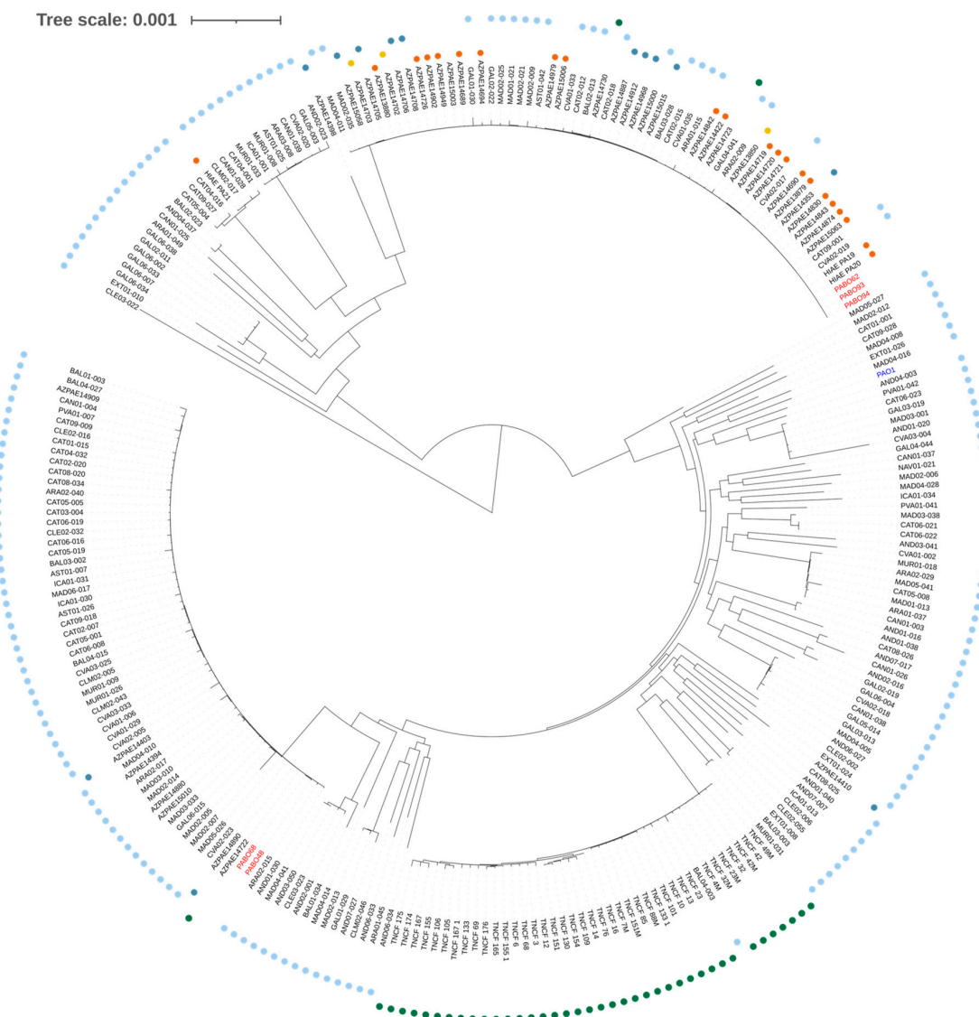
Figure 4. Maximum likelihood phylogeny based on the core genome SNP of the Pseudomonas aeruginosa genomes. The P. aeruginosa strains (clinical and environmental isolates) included in this study are written in red font, and the references strain is written in blue font. Yellow circles indicate strains isolated in Asia, orange circles indicate strains isolated from North and South America, light blue circles indicate strains isolated from Spain, green circles indicate strains isolated from Italy, and dark blue circles indicate strains isolated from other European Union countries.
