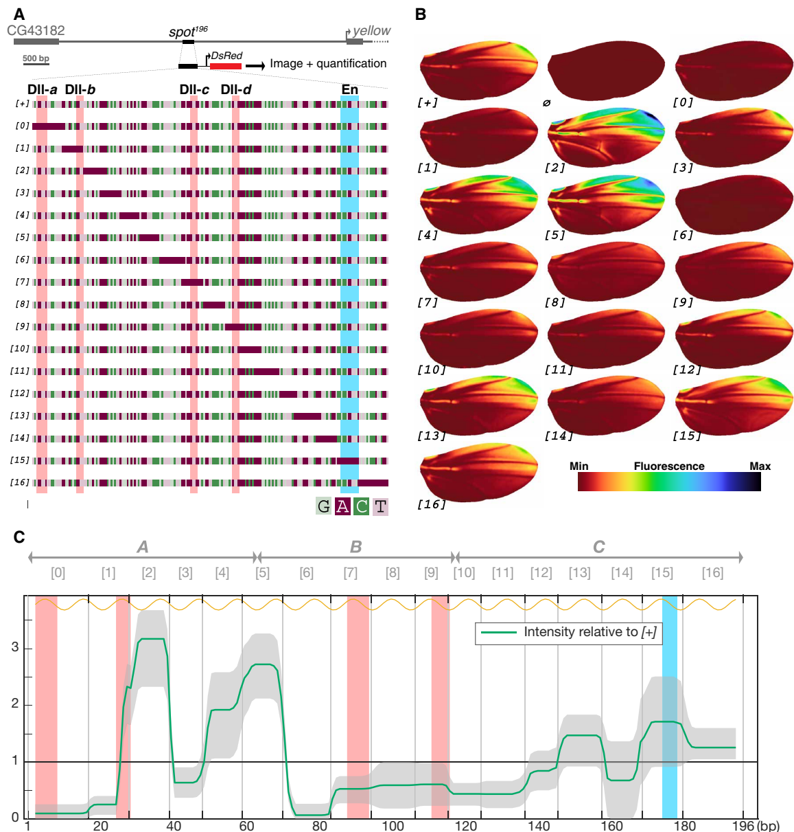
Fig. 1. A mutational scan of the D. biarmipes spot^{196} enhancer with a quantitative reporter assay. (A) Wild-type (+) and mutant ([0] to [16]) versions of the spot^{196} enhancer from the D. biarmipes yellow locus (depicted at the top) were cloned upstream of a DsRed reporter to assay their respective activities in transgenic D. melanogaster . Each mutant targets a position of the enhancer, where the native sequence was replaced by an A-tract (color code: light green, guanine; purple, adenine; dark green, cytosine; pink, thymine). Four characterized binding sites for the TF Distal-less (DII-a, DII-b, DII-c, and DII-d) (19) are highlighted in red, and a single binding site for the TF Engrailed (20) is highlighted in blue across all constructs. (B) Average wing reporter expression for each construct depicted in (A) and an empty reporter vector ( \emptyset ). Each wing image is produced from 11 to 77 individual wing images (38 on average; data file S2), aligned onto a unique wing model. The average image is smoothed, and intensity levels are indicated by a colormap. (C) Mutational effect on intensity of activity along the spot^{196} sequence. The phenotypic effect of each mutation described in (A) along the spot^{196} sequence (x axis) is plotted as the average level of expression across the wing relative to the wild-type average levels. Shaded gray areas around the curve represent the 95% confidence interval of the average levels per position. "1" on the y axis represents the mean wild-type intensity of reporter expression. The graph shows how each construct departs from the wild-type activity (see Materials and Methods). Mutation positions in constructs [0] to [16] are indicated above the graph. The locations of blocks A, B, and C, analyzed in Fig. 3, are also indicated above the graph. The yellow curve above the graph indicates the helical phasing.
