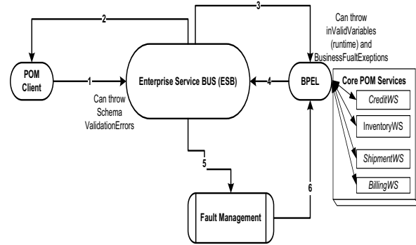
Figure 7: Manageability Usage Scenario
