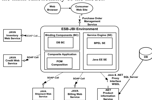
Figure 5: Structure the Case Study
