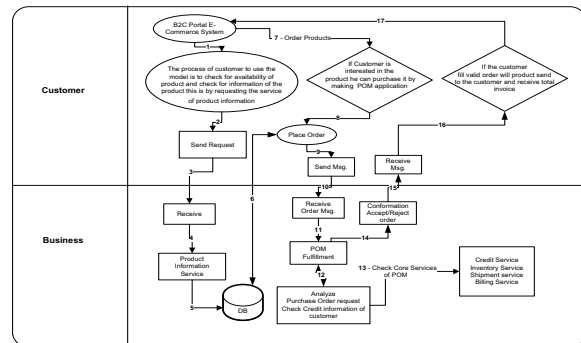
Figure 4: Scenario Workflow Based on the Model
