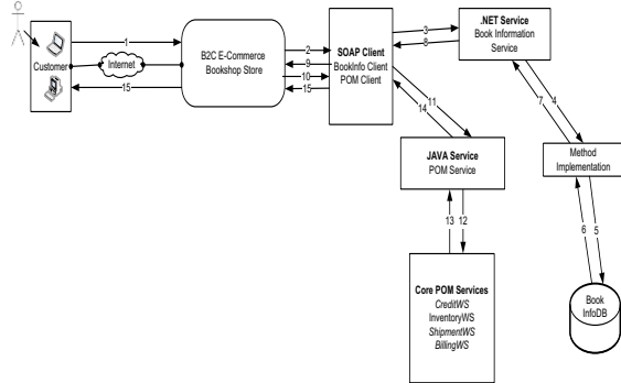
Figure 6: Interoperability Usage Scenario
