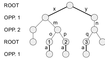
Fig. 2: Opponent Move Abstraction. The root player’s OMA identifies the moves a from nodes 1 and 2, because they have the same history of root player moves, x . The move a from move 3 has a separate OMA value estimate.
