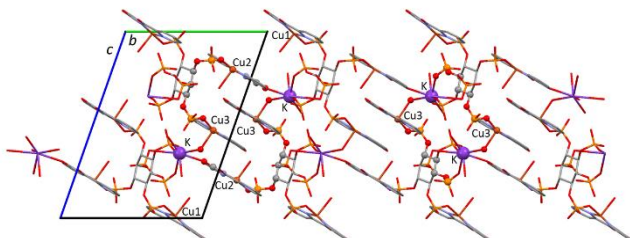
Figure 6. The 1D (\text{K}(\text{H}_2\text{O})_3\{[\text{Cu}(\text{H}_2\text{O})(\text{bpcac})]_3\text{H}_8\text{L}\})_n polymeric coordination chains in 2 growing along the b crystallographic axis (light green arrow). Ball and stick graph is used to evidence the 32-membered and the 24-membered rings. H atoms and co-crystallized water molecules were omitted.
