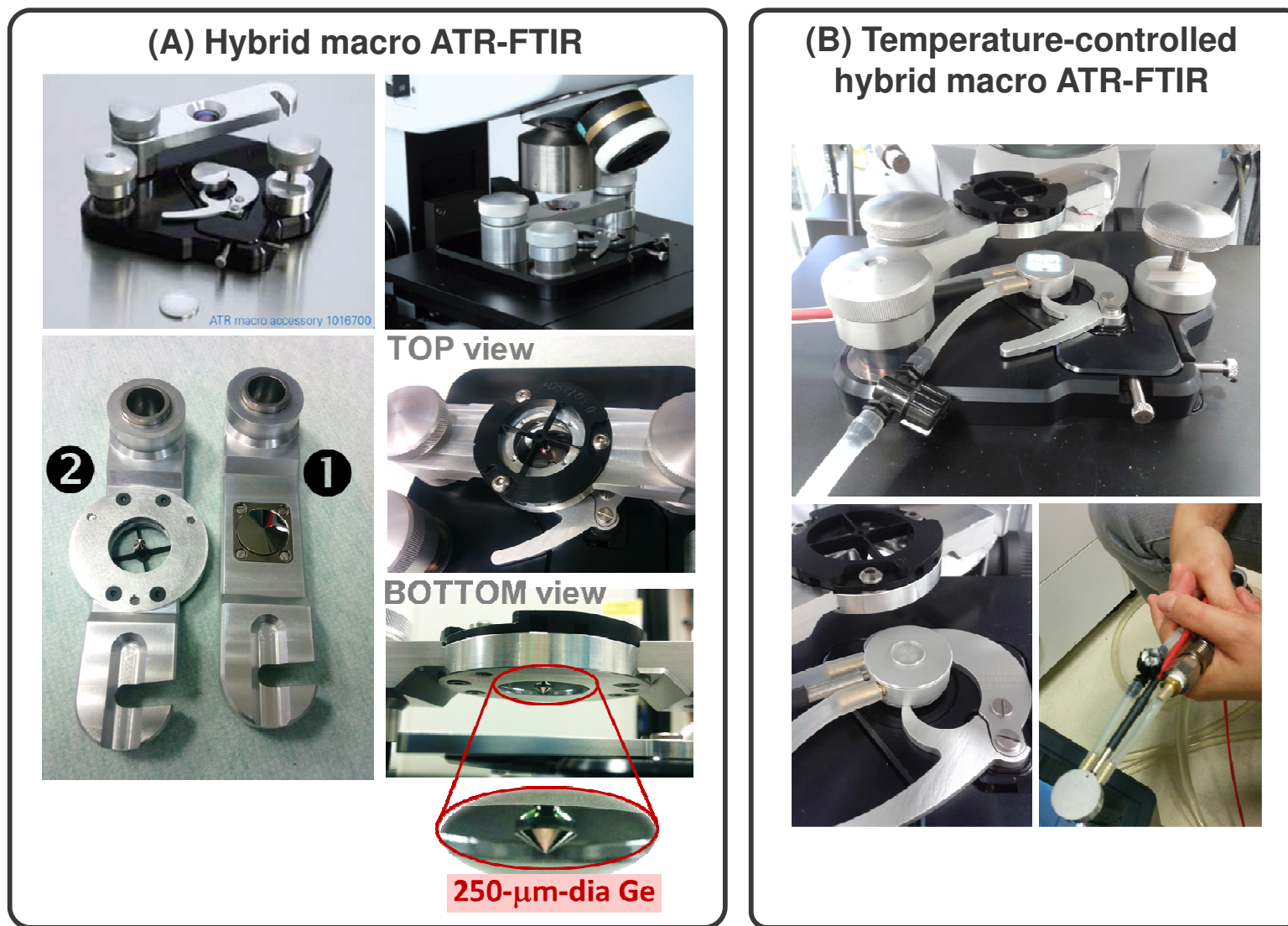
Figure 1. (A) Hybrid macro ATR-FTIR device, showing the standard macro ATR-FTIR unit (top) and the adaptation of cantilever arm to couple with the smaller diameter Ge micro-ATR crystal ②, compared to the original 1 mm diameter Ge macro-ATR crystal ① (bottom). (B) Modification of the sample stage to couple with a temperature control unit, allowing water circulation for temperature-dependent studies.
