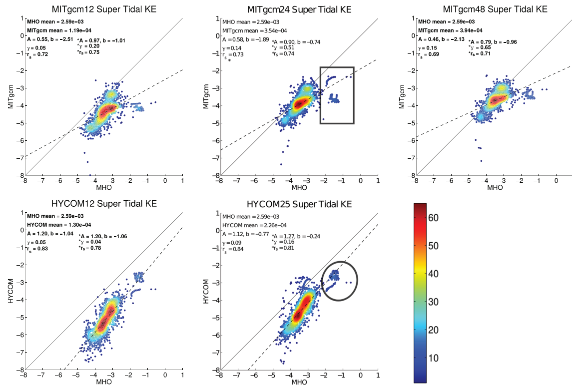
Figure 5. A point-to-point comparison of supertidal kinetic energy [ \log_{10}(\text{m}^2 \text{ s}^{-2}) ] between model and MHO. The top panels show MITgcm12, MITgcm24, and MITgcm48, while the bottom panels show HYCOM12 and HYCOM25. Population density is given by color, with the most tightly grouped data shown in red and the sparsest data in blue. The one-to-one line is shown in solid black, and the linear regression is shown as a dashed line. Spatial means of MHO and model values, and statistical metrics A , b , \gamma , and r_s between each model and the MHO data, are printed on the upper left of each subplot. The second, rightmost, statistical values, marked with an asterisk, are computed after the anomalous high-velocity values, enclosed by a box in the MITgcm24 subplot and an ellipse in the HYCOM25 subplot, have been removed.
